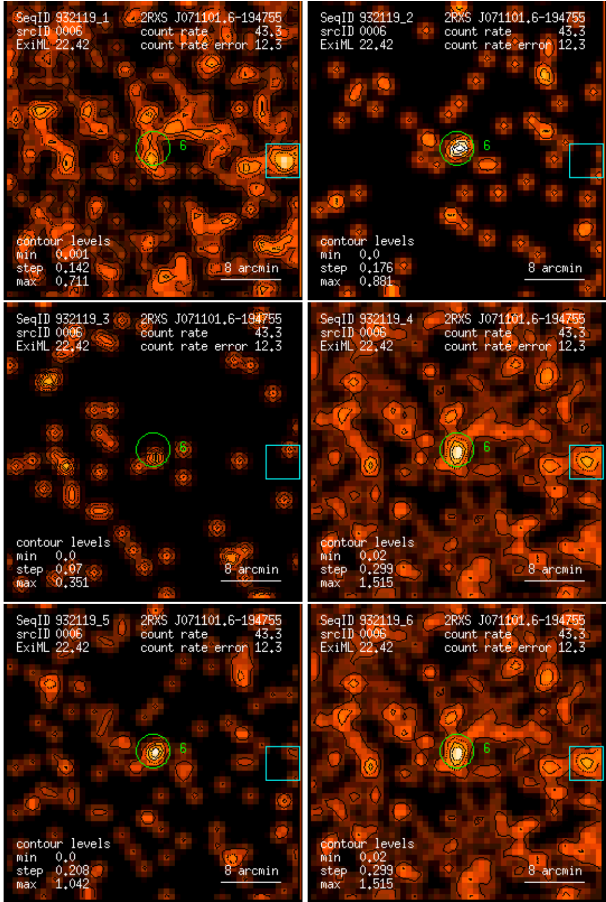
Figure 6: RASS 932119: detection 0006: band rate images, Gaussian filter: (1) PSPC channels 11 – 41, (2) 52 – 90, (3) 91 – 201, (4) 11 – 235, (5) 52 – 201, (6) 11 – 201. Broad band rates in counts/ks. Band rate contour levels in counts/ks/arcmin 2 .
