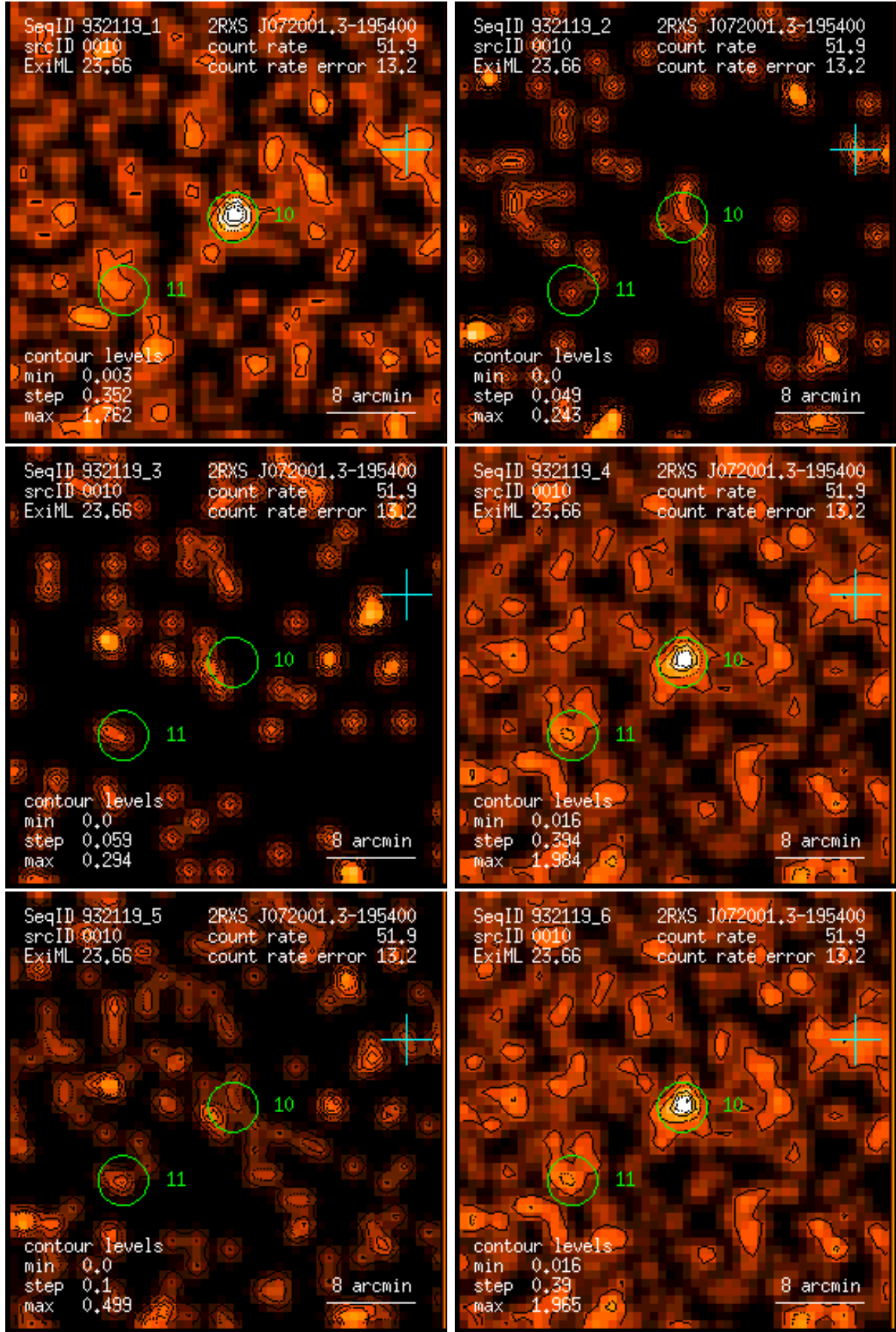
Figure 10: RASS 932119: detection 0010: band rate images, Gaussian filter: (1) PSPC channels 11 – 41, (2) 52 – 90, (3) 91 – 201, (4) 11 – 235, (5) 52 – 201, (6) 11 – 201. Broad band rates in counts/ks. Band rate contour levels in counts/ks/arcmin 2 .
