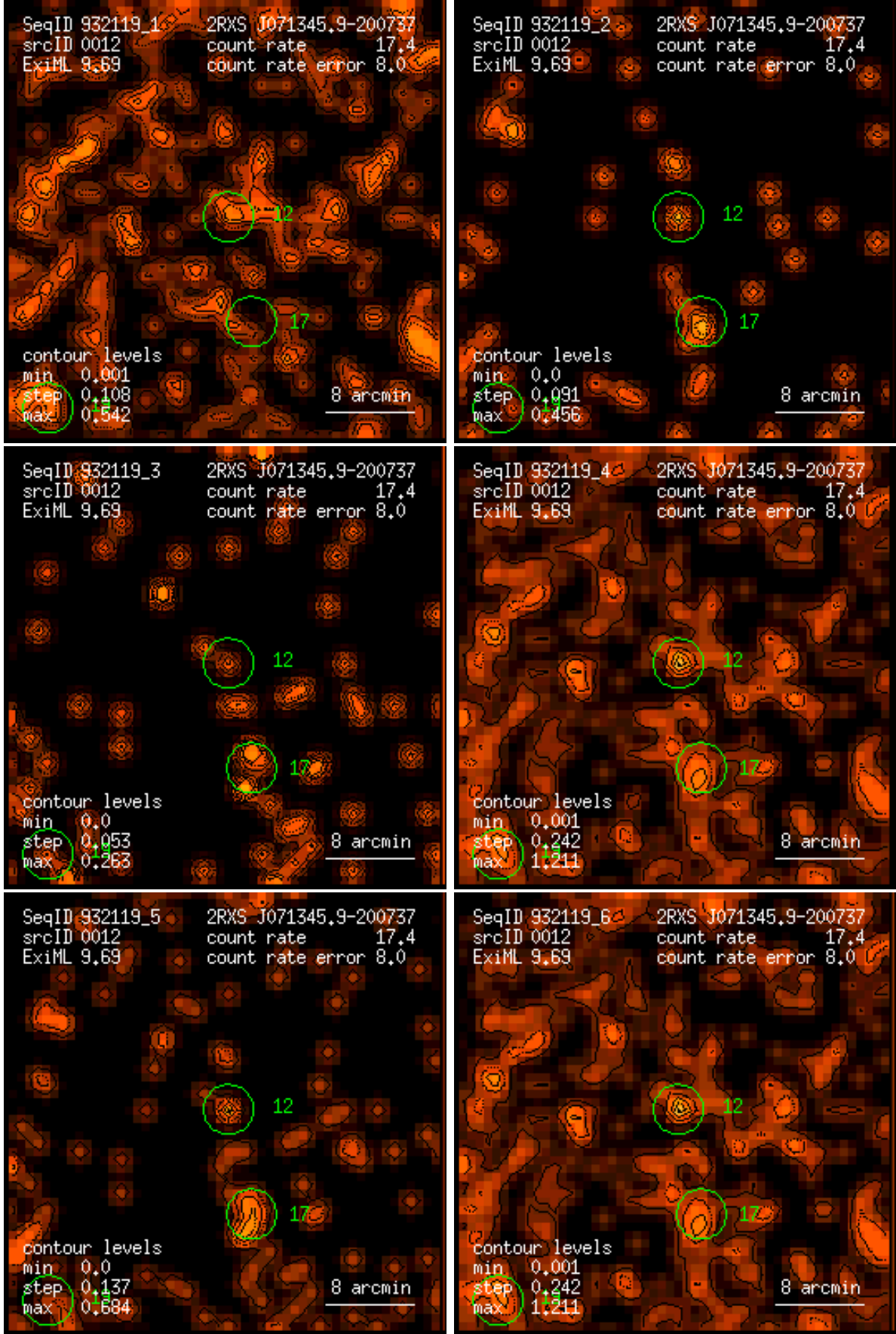
Figure 12: RASS 932119: detection 0012: band rate images, Gaussian filter: (1) PSPC channels 11 – 41, (2) 52 – 90, (3) 91 – 201, (4) 11 – 235, (5) 52 – 201, (6) 11 – 201. Broad band rates in counts/ks. Band rate contour levels in counts/ks/arcmin 2 .
