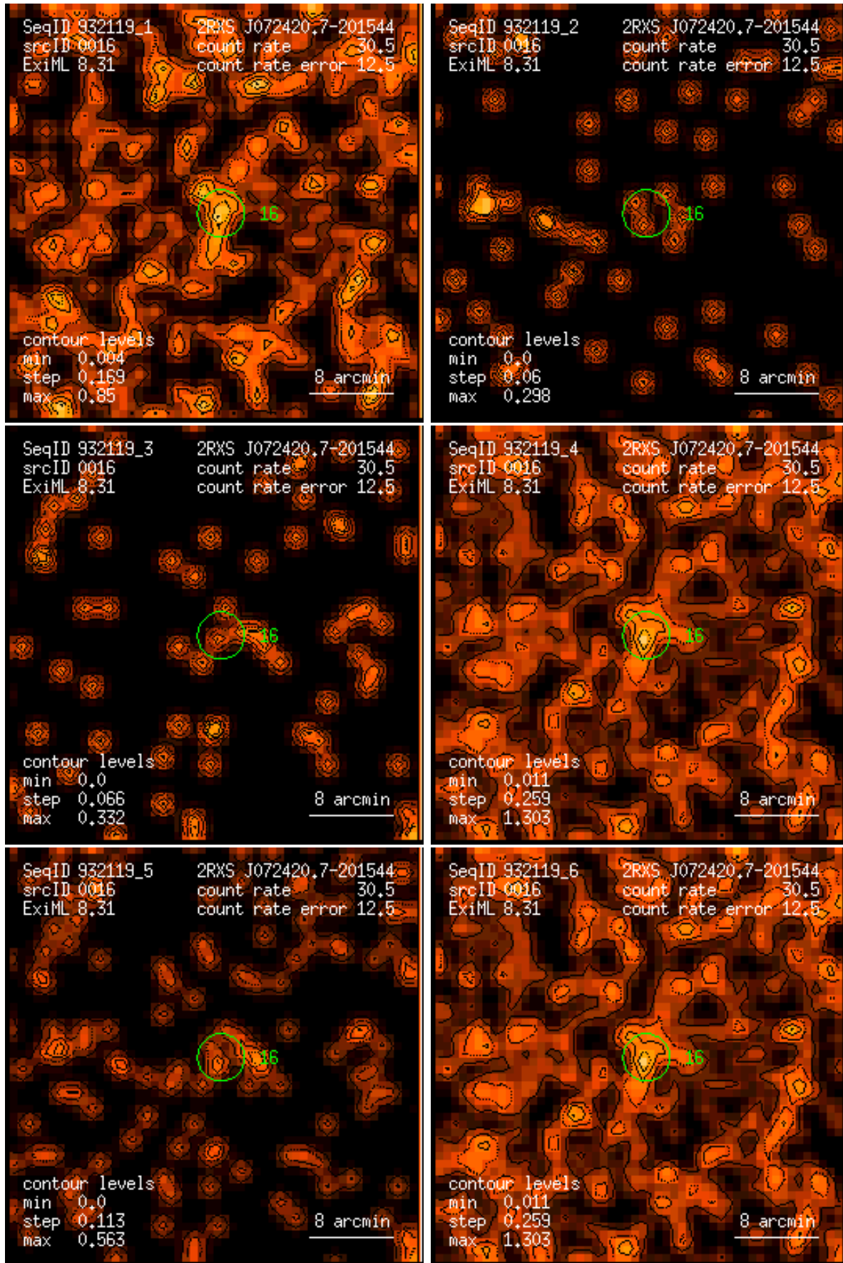
Figure 16: RASS 932119: detection 0016: band rate images, Gaussian filter: (1) PSPC channels 11 – 41, (2) 52 – 90, (3) 91 – 201, (4) 11 – 235, (5) 52 – 201, (6) 11 – 201. Broad band rates in counts/ks. Band rate contour levels in counts/ks/arcmin 2 .
