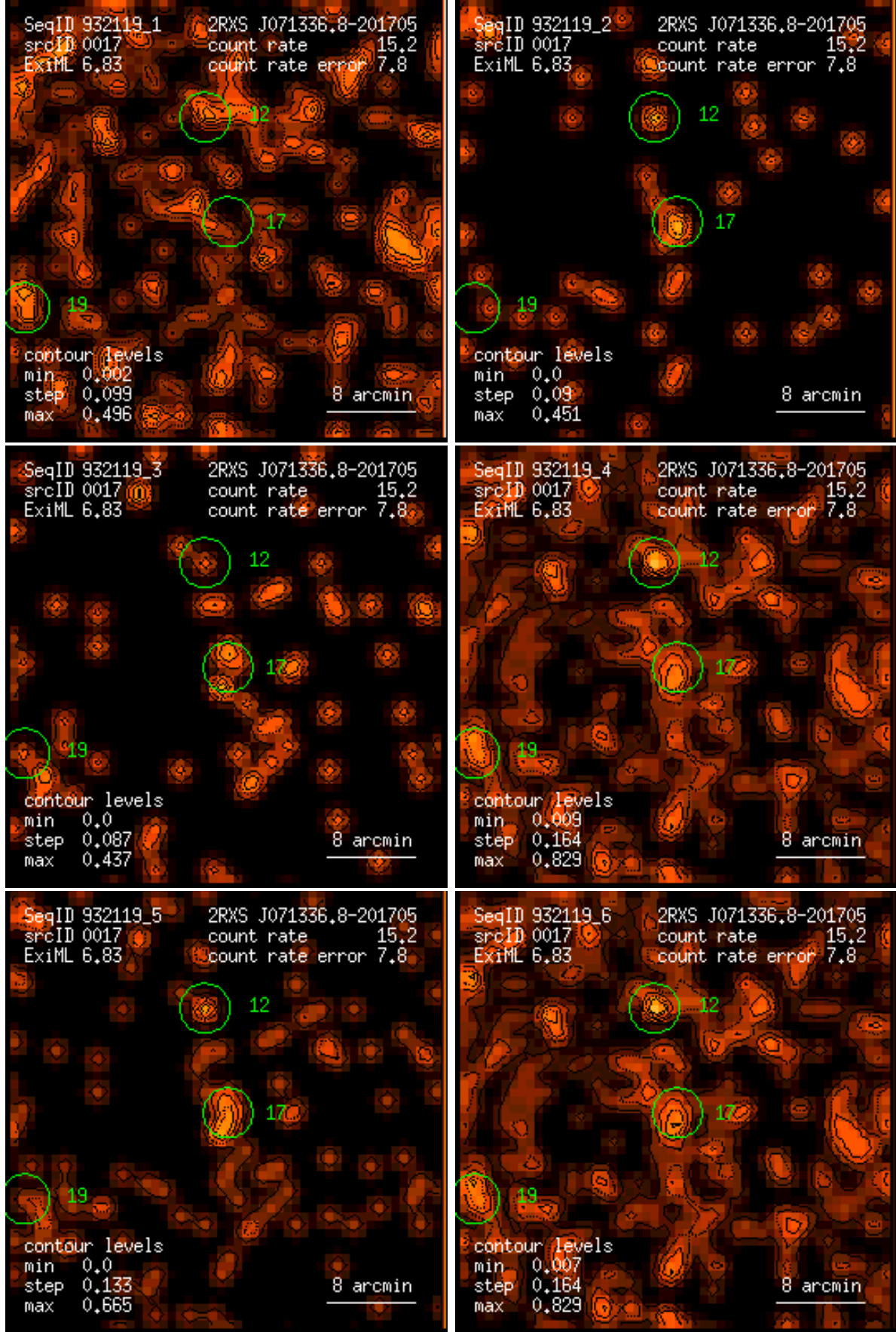
Figure 17: RASS 932119: detection 0017: band rate images, Gaussian filter: (1) PSPC channels 11 – 41, (2) 52 – 90, (3) 91 – 201, (4) 11 – 235, (5) 52 – 201, (6) 11 – 201. Broad band rates in counts/ks. Band rate contour levels in counts/ks/arcmin 2 .
