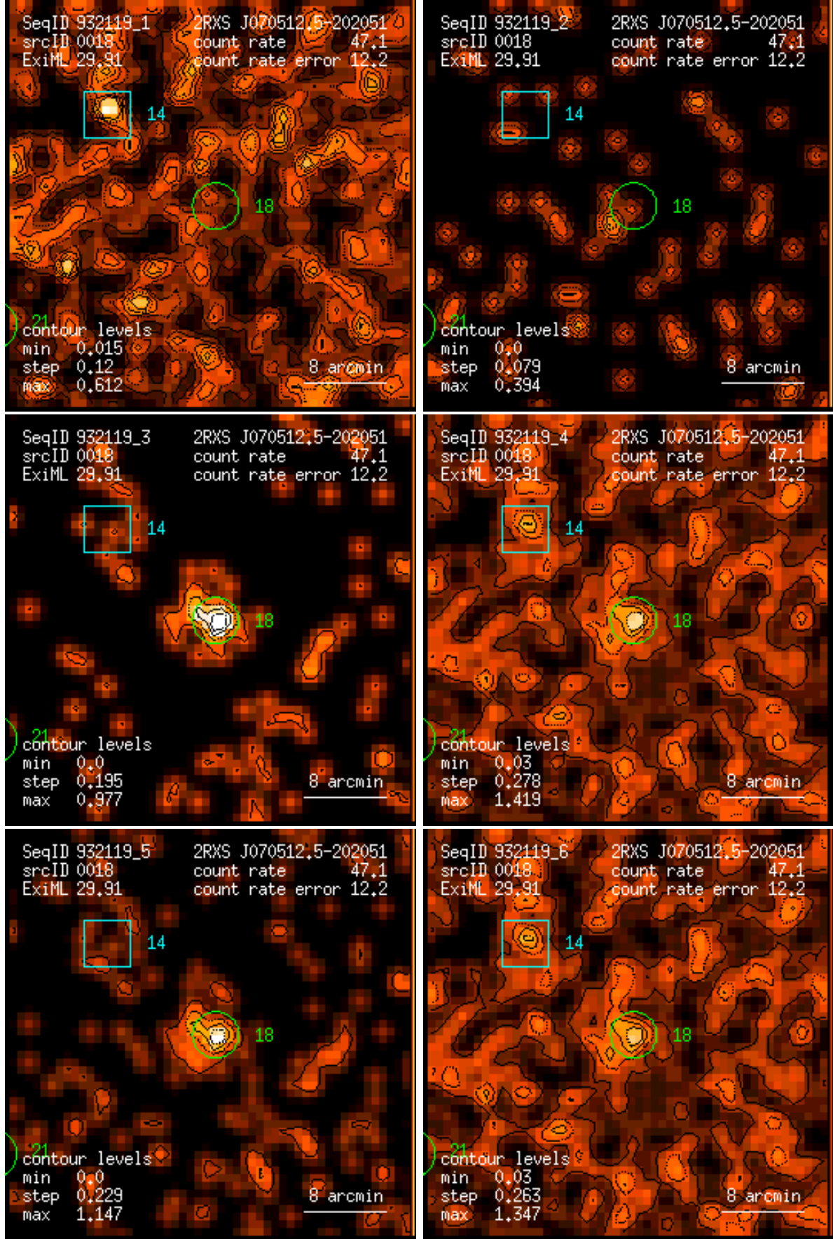
Figure 18: RASS 932119: detection 0018: band rate images, Gaussian filter: (1) PSPC channels 11 – 41, (2) 52 – 90, (3) 91 – 201, (4) 11 – 235, (5) 52 – 201, (6) 11 – 201. Broad band rates in counts/ks. Band rate contour levels in counts/ks/arcmin 2 .
