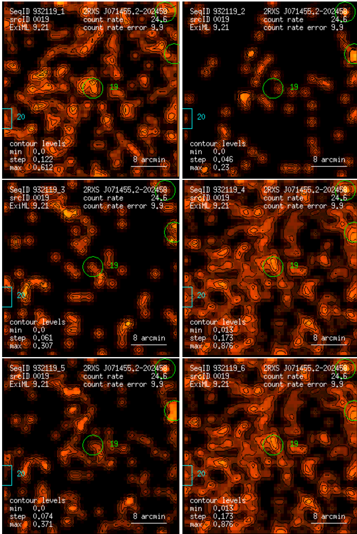
Figure 19: RASS 932119: detection 0019: band rate images, Gaussian filter: (1) PSPC channels 11 – 41, (2) 52 – 90, (3) 91 – 201, (4) 11 – 235, (5) 52 – 201, (6) 11 – 201. Broad band rates in counts/ks. Band rate contour levels in counts/ks/arcmin 2 .
