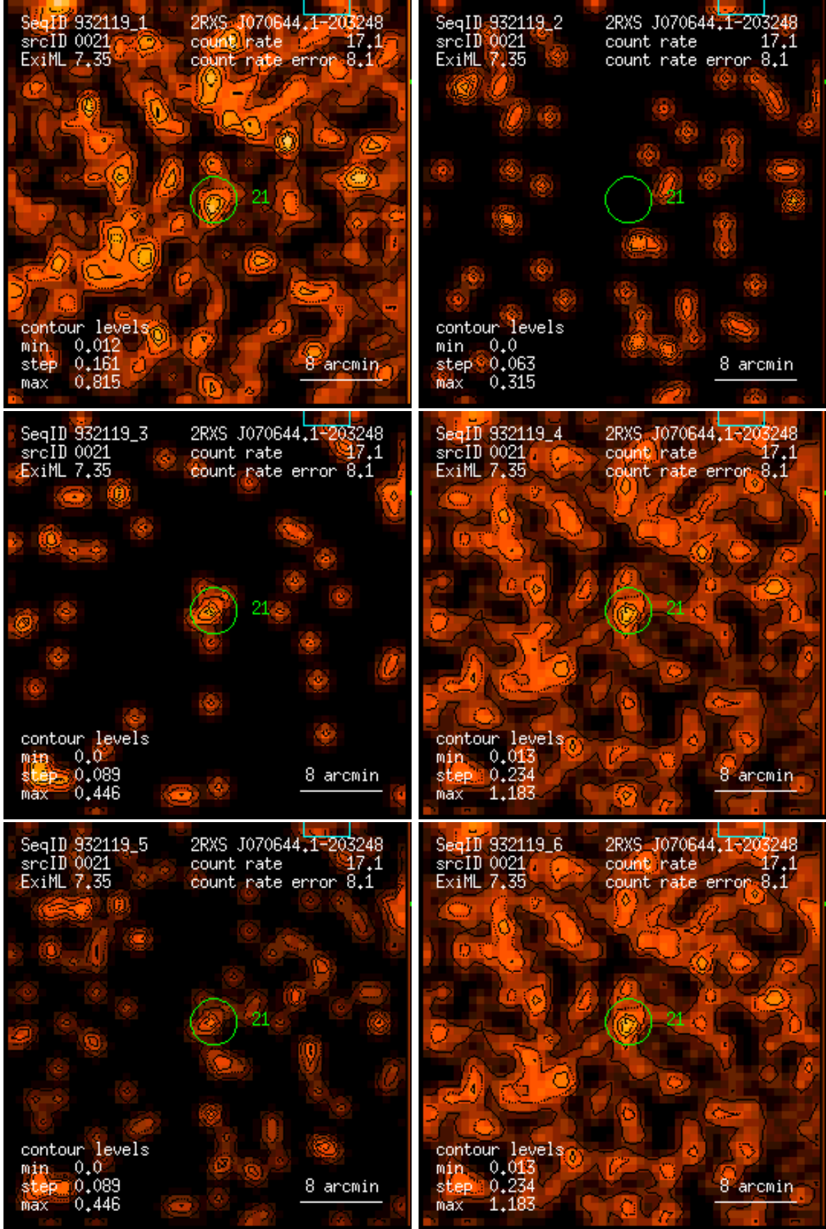
Figure 21: RASS 932119: detection 0021: band rate images, Gaussian filter: (1) PSPC channels 11 – 41, (2) 52 – 90, (3) 91 – 201, (4) 11 – 235, (5) 52 – 201, (6) 11 – 201. Broad band rates in counts/ks. Band rate contour levels in counts/ks/arcmin 2 .
