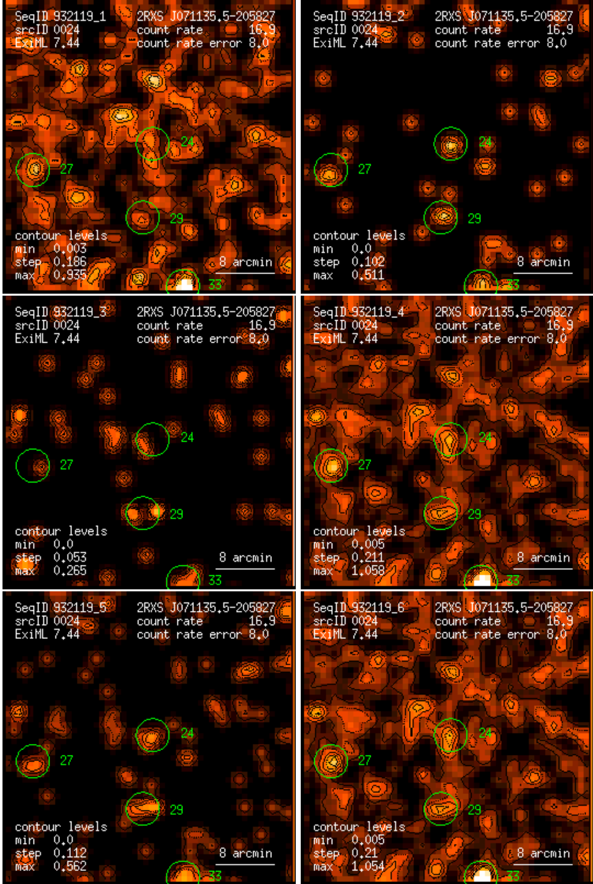
Figure 24: RASS 932119: detection 0024: band rate images, Gaussian filter: (1) PSPC channels 11 – 41, (2) 52 – 90, (3) 91 – 201, (4) 11 – 235, (5) 52 – 201, (6) 11 – 201. Broad band rates in counts/ks. Band rate contour levels in counts/ks/arcmin 2 .
