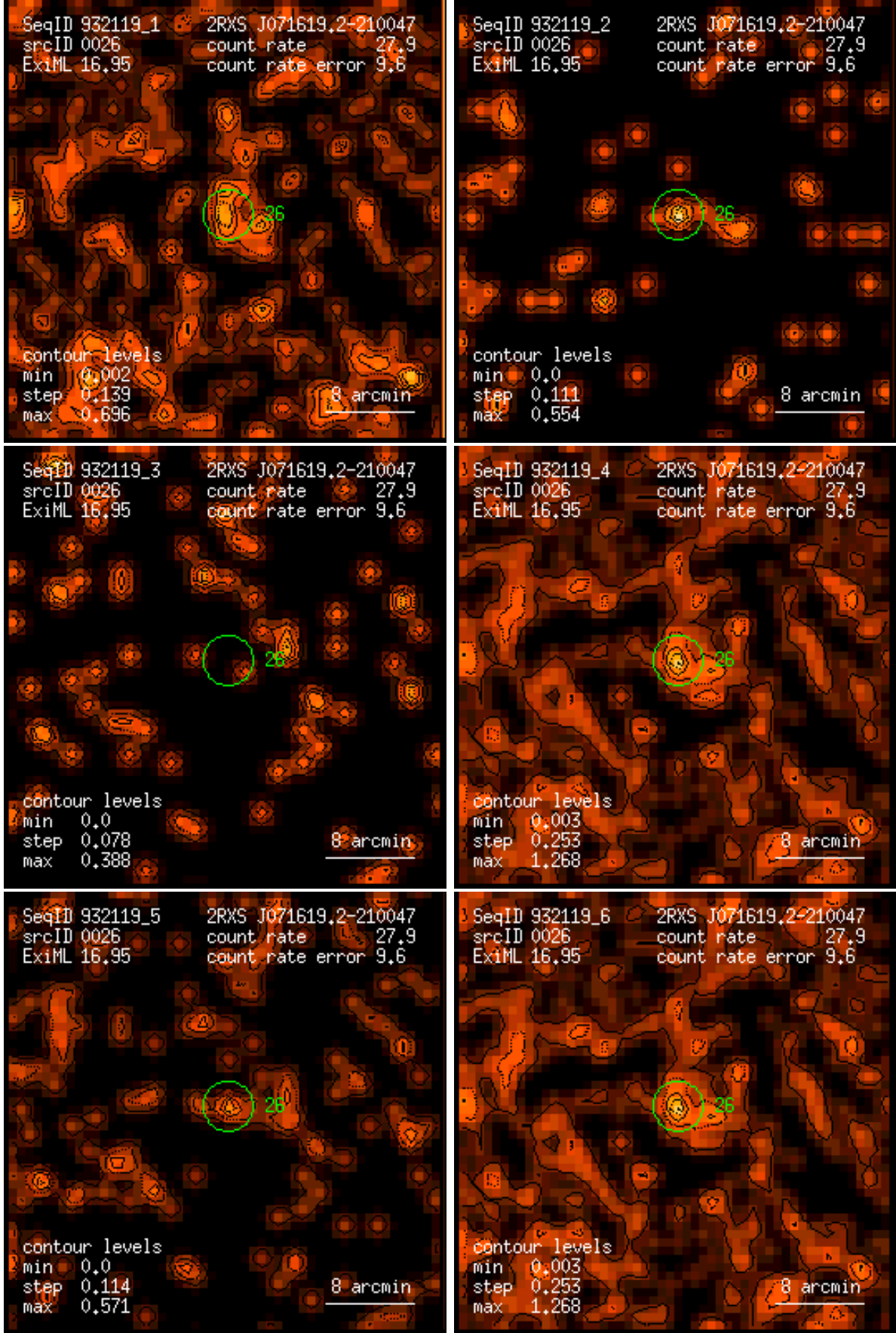
Figure 26: RASS 932119: detection 0026: band rate images, Gaussian filter: (1) PSPC channels 11 – 41, (2) 52 – 90, (3) 91 – 201, (4) 11 – 235, (5) 52 – 201, (6) 11 – 201. Broad band rates in counts/ks. Band rate contour levels in counts/ks/arcmin 2 .
