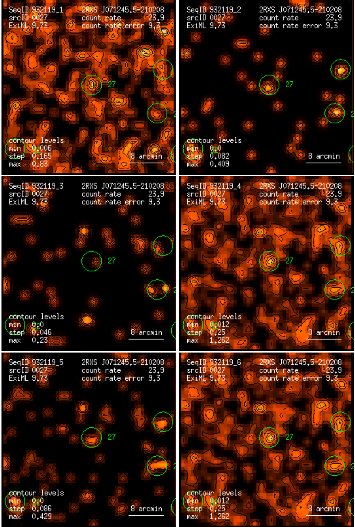
Figure 27: RASS 932119: detection 0027: band rate images, Gaussian filter: (1) PSPC channels 11 – 41, (2) 52 – 90, (3) 91 – 201, (4) 11 – 235, (5) 52 – 201, (6) 11 – 201. Broad band rates in counts/ks. Band rate contour levels in counts/ks/arcmin 2 .
