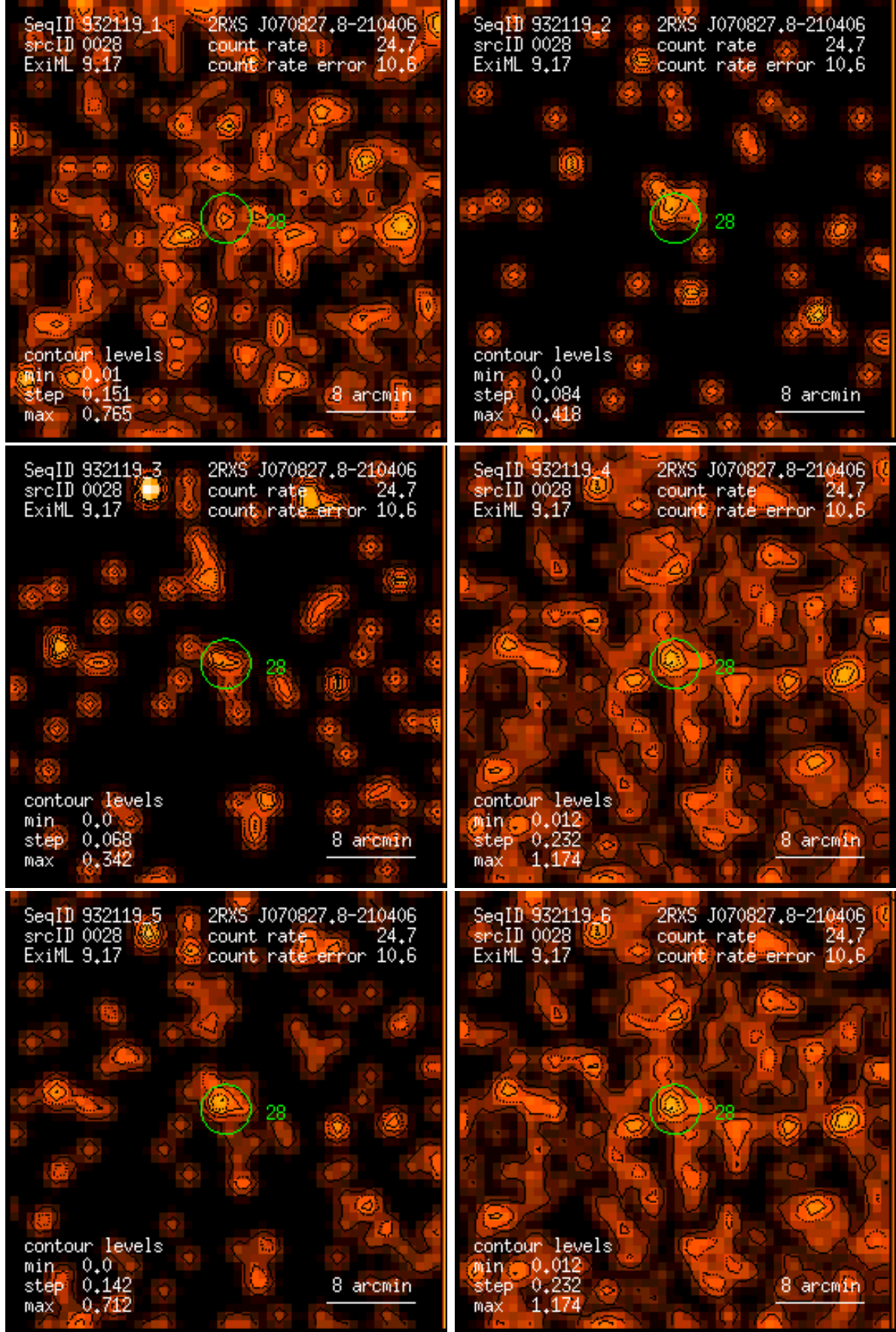
Figure 28: RASS 932119: detection 0028: band rate images, Gaussian filter: (1) PSPC channels 11 – 41, (2) 52 – 90, (3) 91 – 201, (4) 11 – 235, (5) 52 – 201, (6) 11 – 201. Broad band rates in counts/ks. Band rate contour levels in counts/ks/arcmin 2 .
