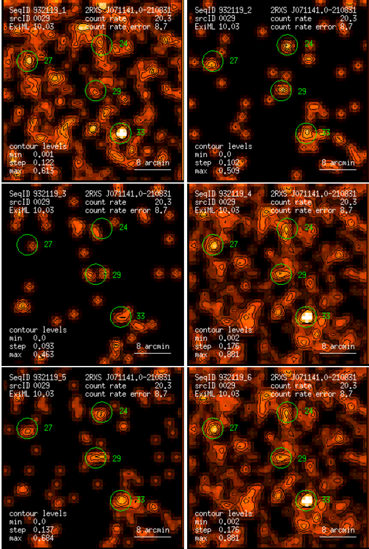
Figure 29: RASS 932119: detection 0029: band rate images, Gaussian filter: (1) PSPC channels 11 – 41, (2) 52 – 90, (3) 91 – 201, (4) 11 – 235, (5) 52 – 201, (6) 11 – 201. Broad band rates in counts/ks. Band rate contour levels in counts/ks/arcmin 2 .
