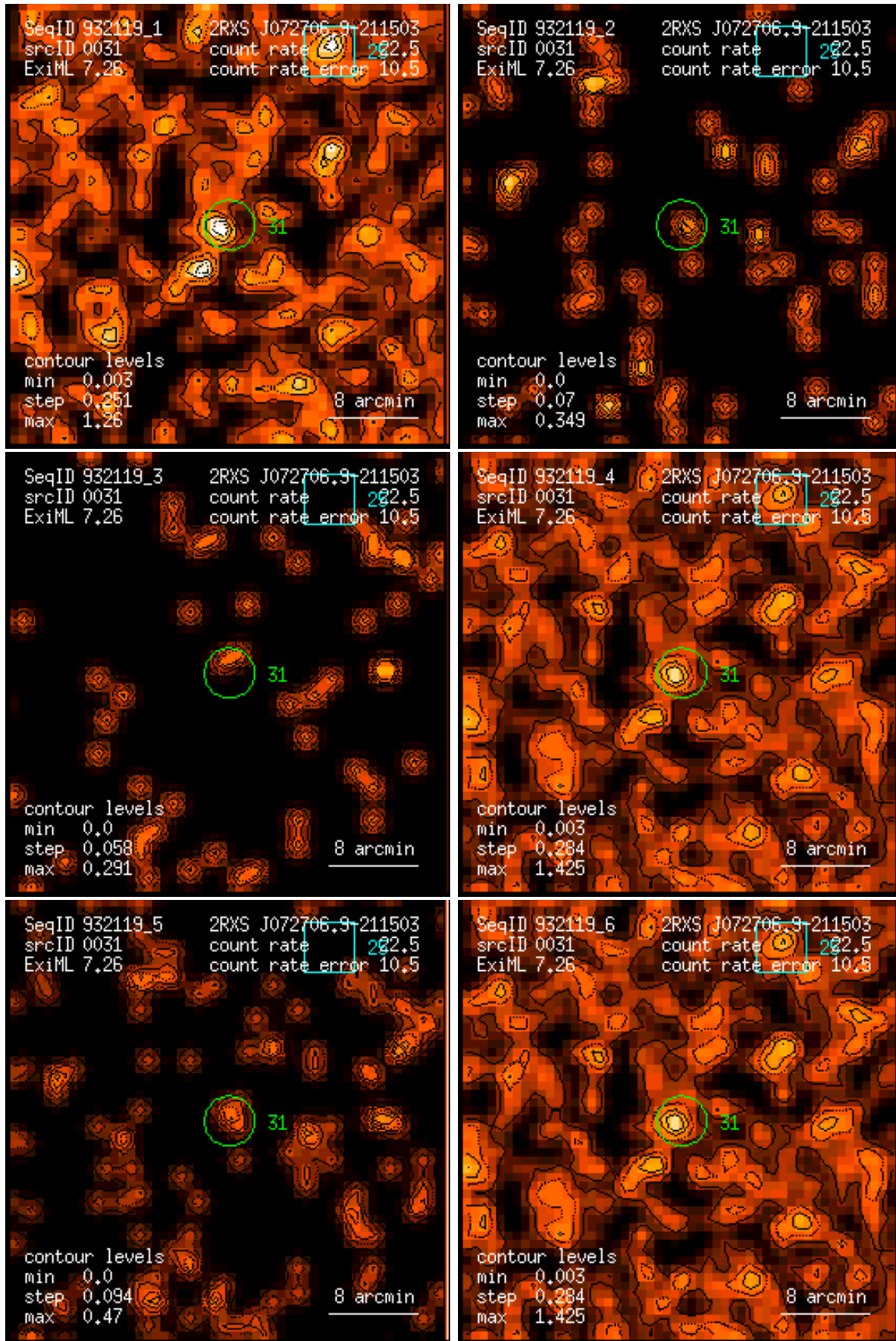
Figure 31: RASS 932119: detection 0031: band rate images, Gaussian filter: (1) PSPC channels 11 – 41, (2) 52 – 90, (3) 91 – 201, (4) 11 – 235, (5) 52 – 201, (6) 11 – 201. Broad band rates in counts/ks. Band rate contour levels in counts/ks/arcmin 2 .
