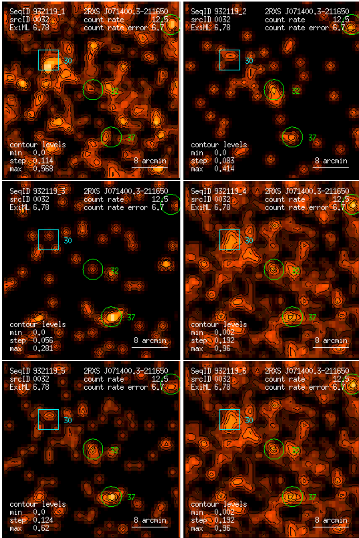
Figure 32: RASS 932119: detection 0032: band rate images, Gaussian filter: (1) PSPC channels 11 – 41, (2) 52 – 90, (3) 91 – 201, (4) 11 – 235, (5) 52 – 201, (6) 11 – 201. Broad band rates in counts/ks. Band rate contour levels in counts/ks/arcmin 2 .
