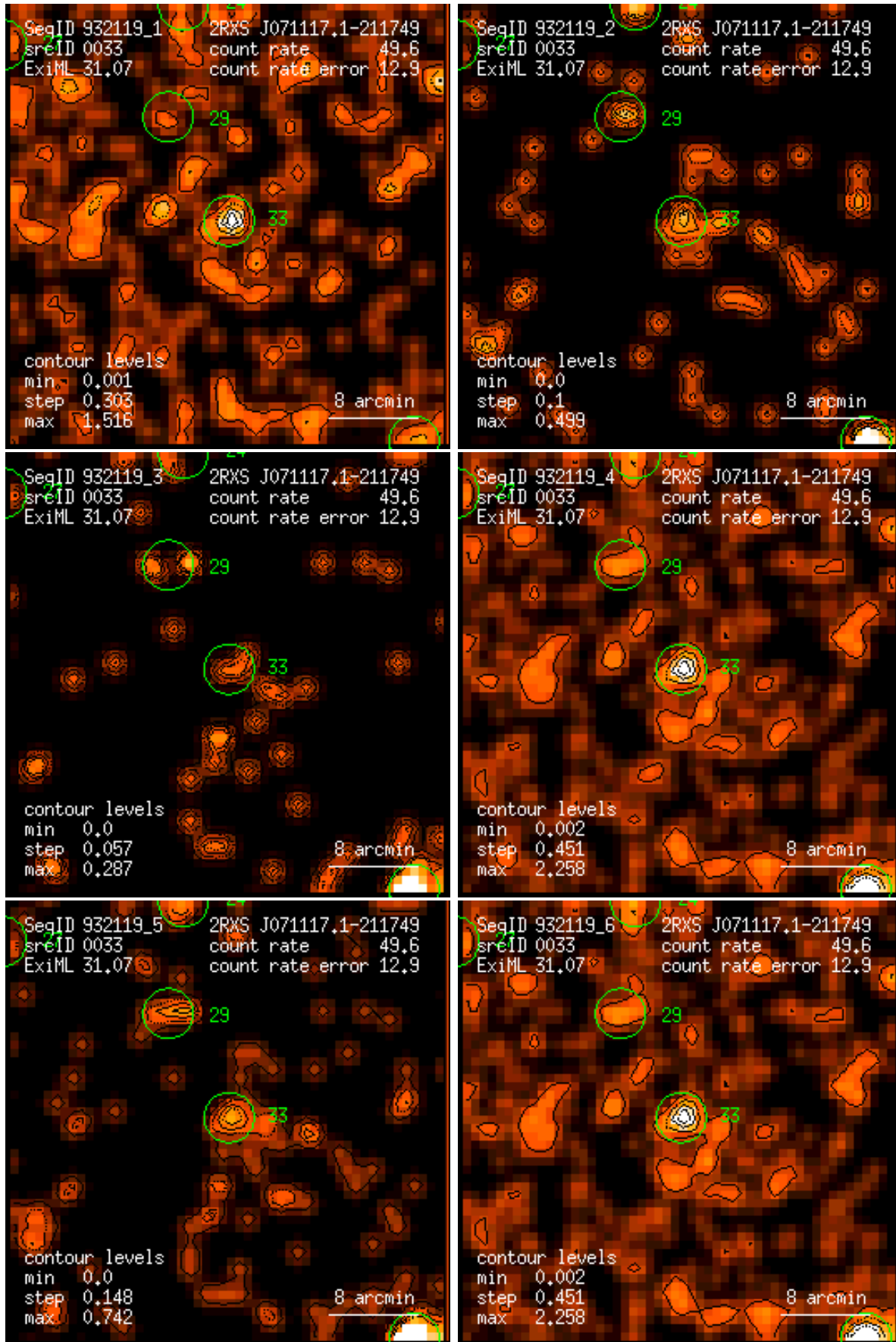
Figure 33: RASS 932119: detection 0033: band rate images, Gaussian filter: (1) PSPC channels 11 – 41, (2) 52 – 90, (3) 91 – 201, (4) 11 – 235, (5) 52 – 201, (6) 11 – 201. Broad band rates in counts/ks. Band rate contour levels in counts/ks/arcmin 2 .
