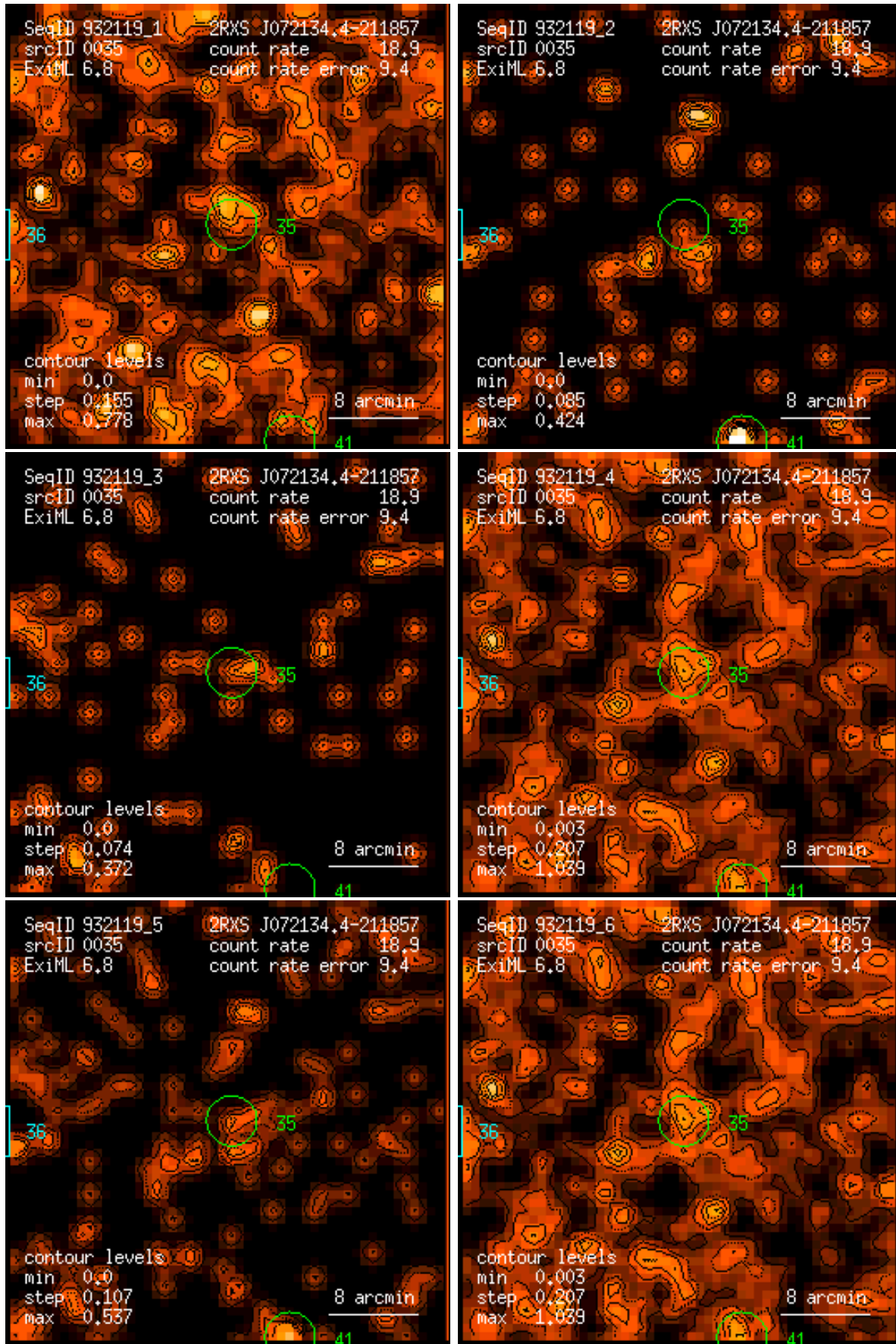
Figure 35: RASS 932119: detection 0035: band rate images, Gaussian filter: (1) PSPC channels 11 – 41, (2) 52 – 90, (3) 91 – 201, (4) 11 – 235, (5) 52 – 201, (6) 11 – 201. Broad band rates in counts/ks. Band rate contour levels in counts/ks/arcmin 2 .
