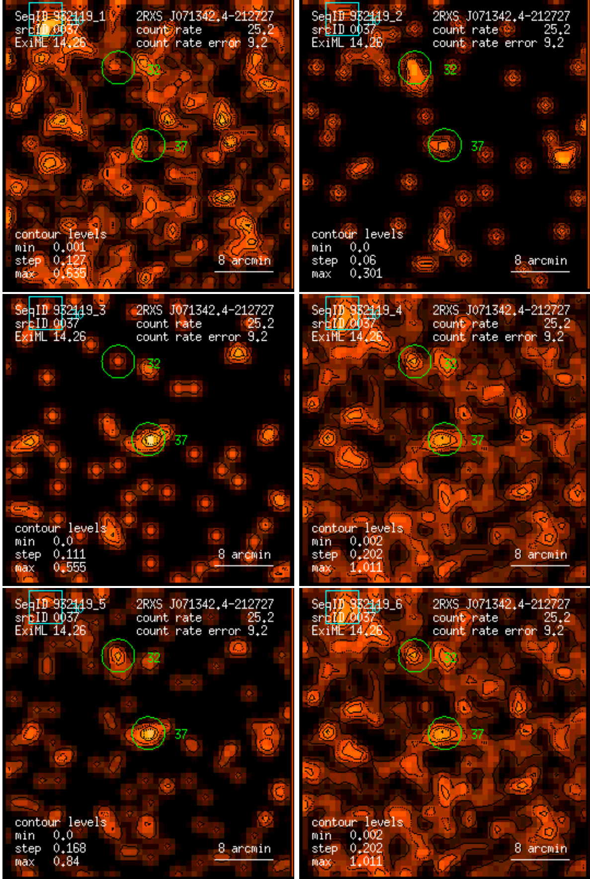
Figure 37: RASS 932119: detection 0037: band rate images, Gaussian filter: (1) PSPC channels 11 – 41, (2) 52 – 90, (3) 91 – 201, (4) 11 – 235, (5) 52 – 201, (6) 11 – 201. Broad band rates in counts/ks. Band rate contour levels in counts/ks/arcmin 2 .
