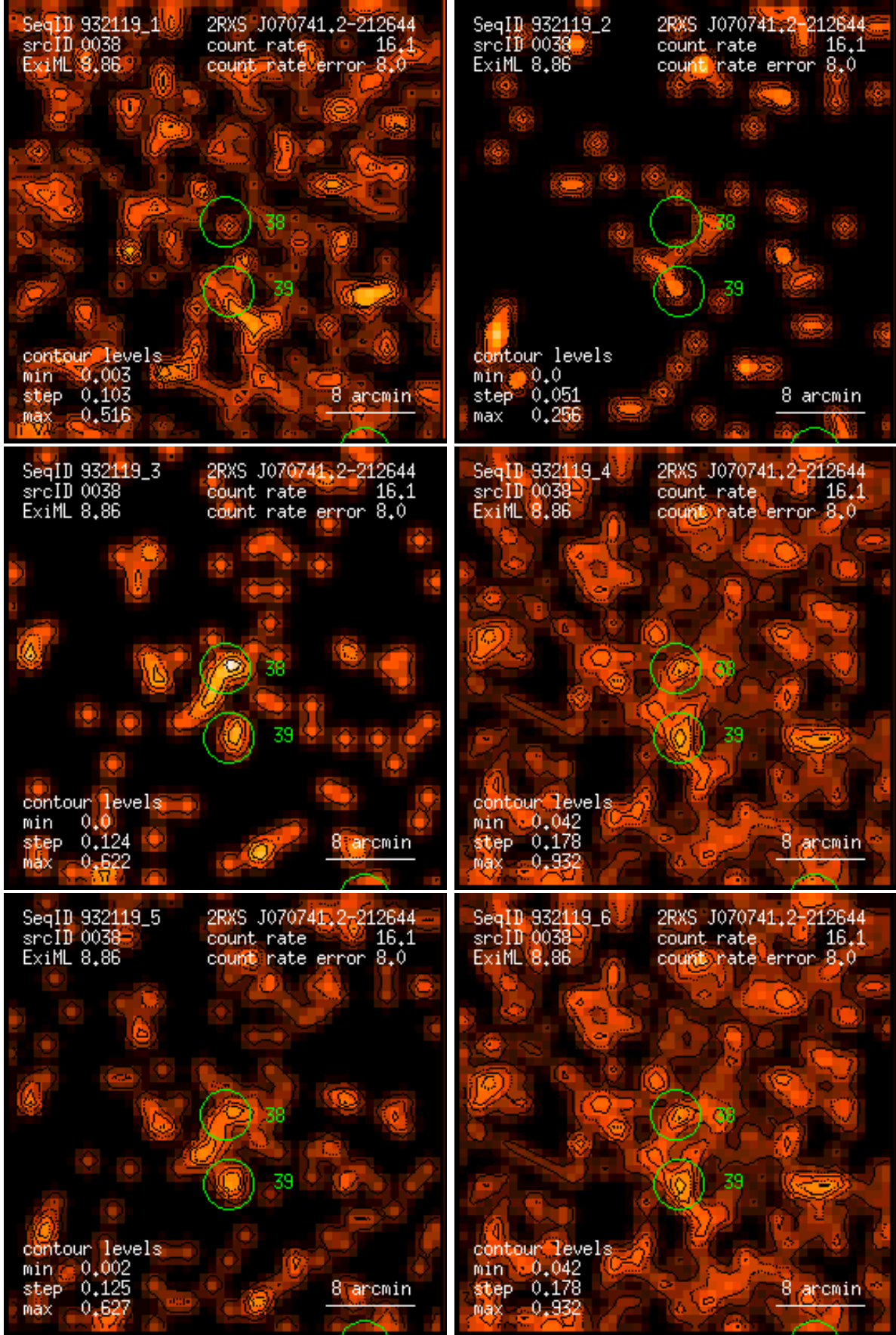
Figure 38: RASS 932119: detection 0038: band rate images, Gaussian filter: (1) PSPC channels 11 – 41, (2) 52 – 90, (3) 91 – 201, (4) 11 – 235, (5) 52 – 201, (6) 11 – 201. Broad band rates in counts/ks. Band rate contour levels in counts/ks/arcmin 2 .
