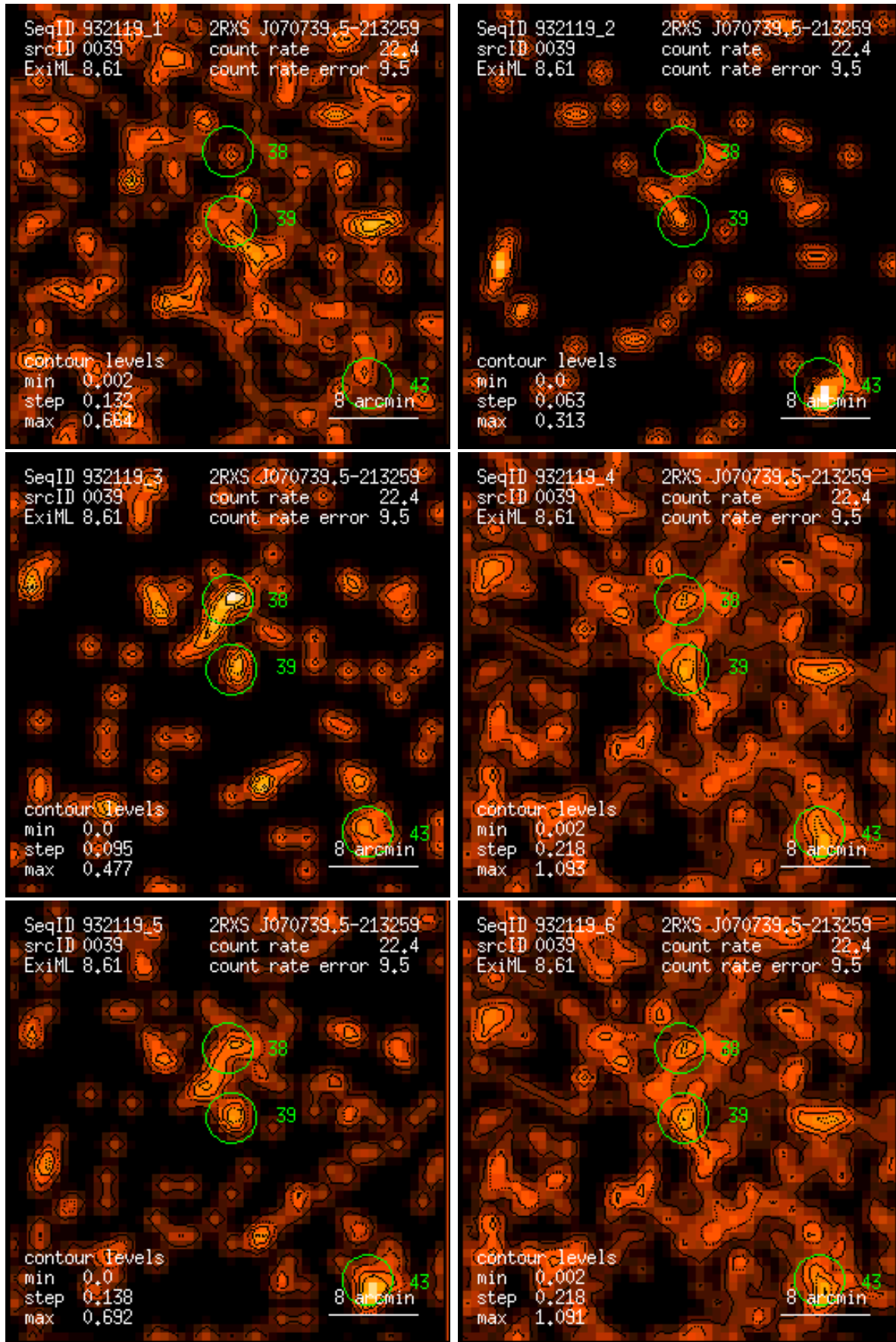
Figure 39: RASS 932119: detection 0039: band rate images, Gaussian filter: (1) PSPC channels 11 – 41, (2) 52 – 90, (3) 91 – 201, (4) 11 – 235, (5) 52 – 201, (6) 11 – 201. Broad band rates in counts/ks. Band rate contour levels in counts/ks/arcmin 2 .
