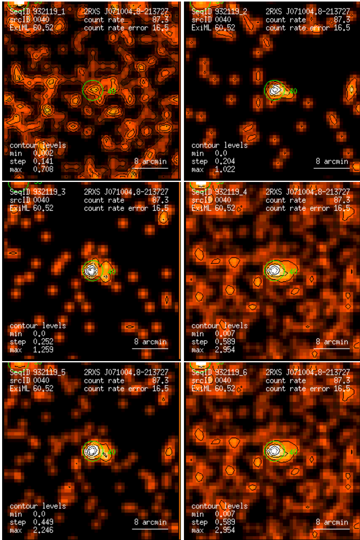
Figure 40: RASS 932119: detection 0040: band rate images, Gaussian filter: (1) PSPC channels 11 – 41, (2) 52 – 90, (3) 91 – 201, (4) 11 – 235, (5) 52 – 201, (6) 11 – 201. Broad band rates in counts/ks. Band rate contour levels in counts/ks/arcmin 2 .
