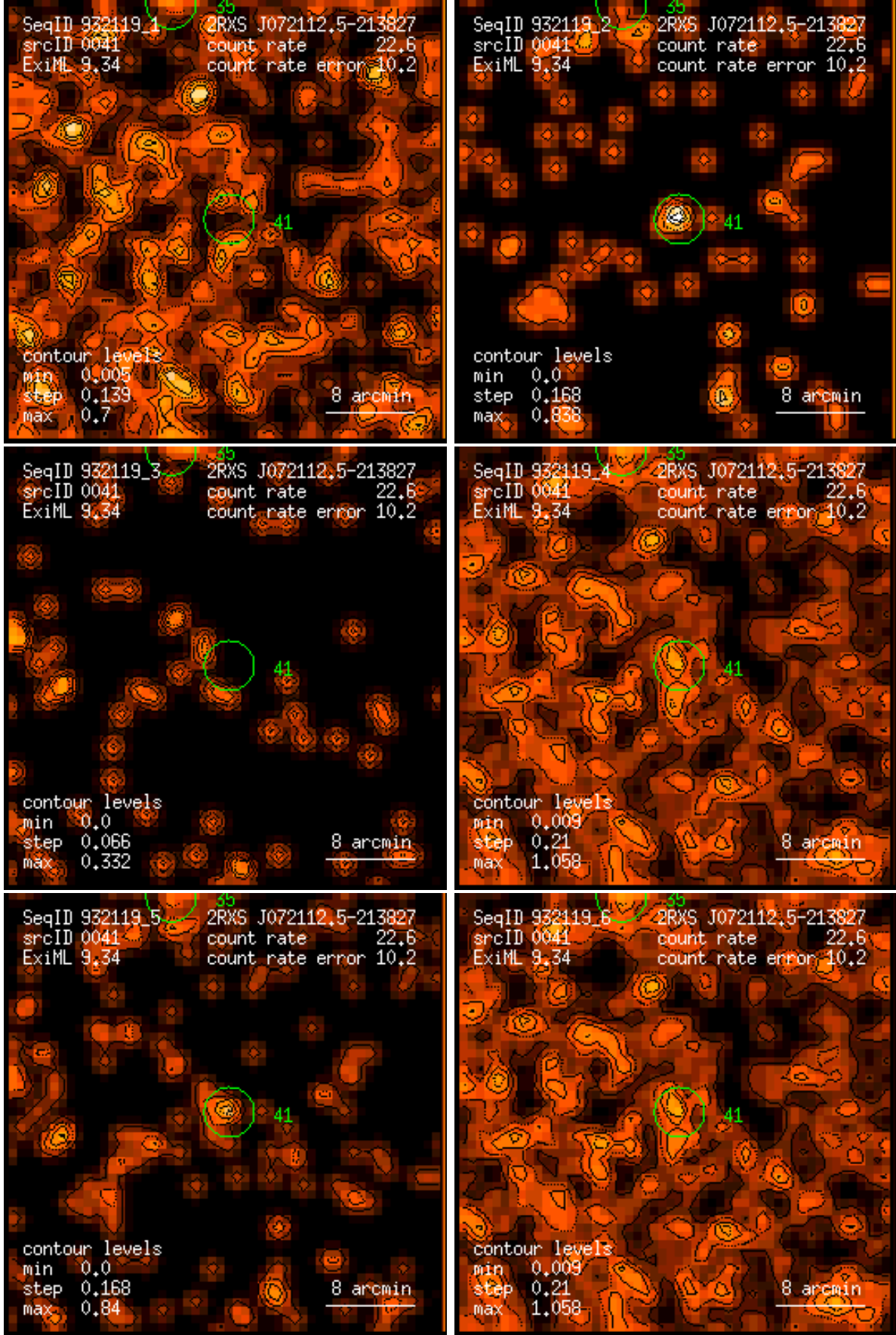
Figure 41: RASS 932119: detection 0041: band rate images, Gaussian filter: (1) PSPC channels 11 – 41, (2) 52 – 90, (3) 91 – 201, (4) 11 – 235, (5) 52 – 201, (6) 11 – 201. Broad band rates in counts/ks. Band rate contour levels in counts/ks/arcmin 2 .
