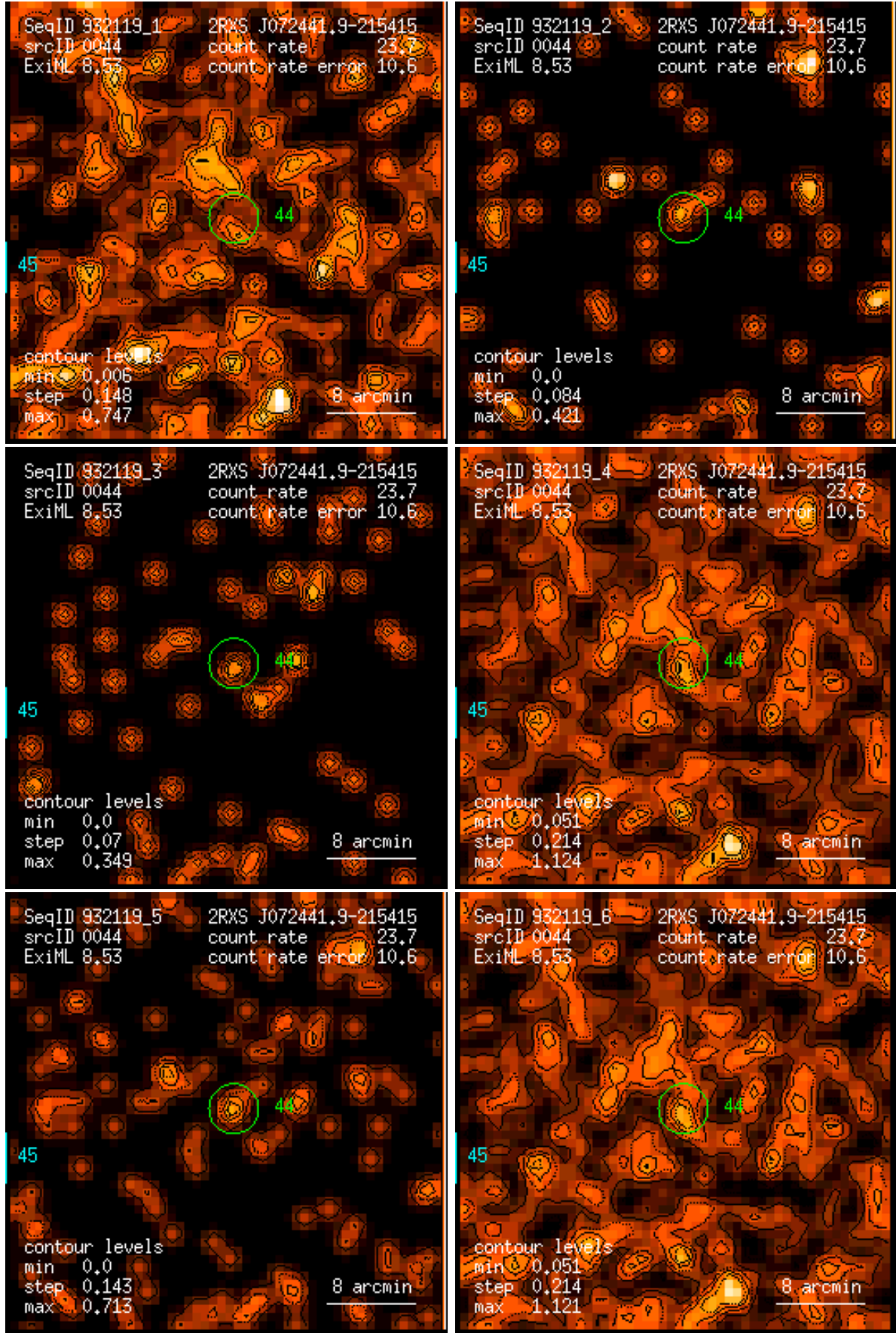
Figure 44: RASS 932119: detection 0044: band rate images, Gaussian filter: (1) PSPC channels 11 – 41, (2) 52 – 90, (3) 91 – 201, (4) 11 – 235, (5) 52 – 201, (6) 11 – 201. Broad band rates in counts/ks. Band rate contour levels in counts/ks/arcmin 2 .
