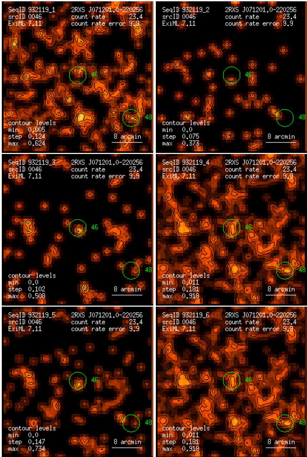
Figure 46: RASS 932119: detection 0046: band rate images, Gaussian filter: (1) PSPC channels 11 – 41, (2) 52 – 90, (3) 91 – 201, (4) 11 – 235, (5) 52 – 201, (6) 11 – 201. Broad band rates in counts/ks. Band rate contour levels in counts/ks/arcmin 2 .
