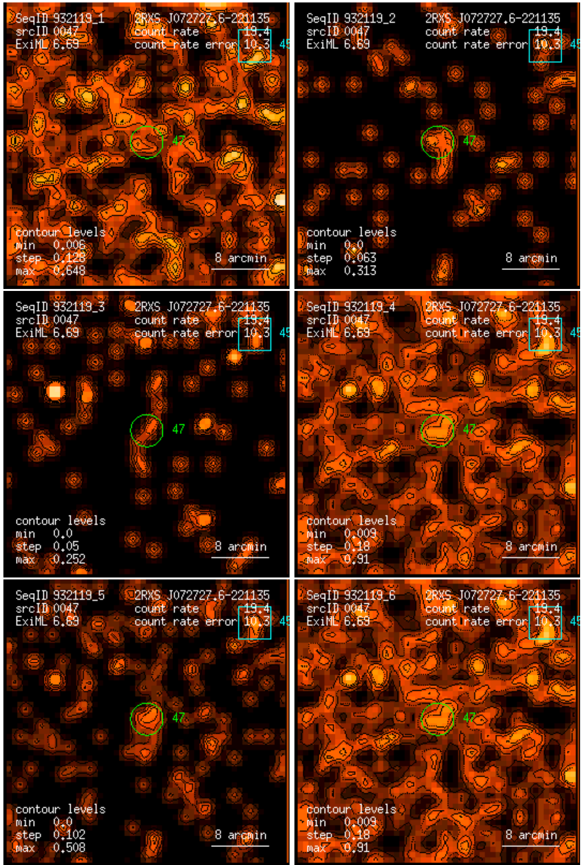
Figure 47: RASS 932119: detection 0047: band rate images, Gaussian filter: (1) PSPC channels 11 – 41, (2) 52 – 90, (3) 91 – 201, (4) 11 – 235, (5) 52 – 201, (6) 11 – 201. Broad band rates in counts/ks. Band rate contour levels in counts/ks/arcmin 2 .
