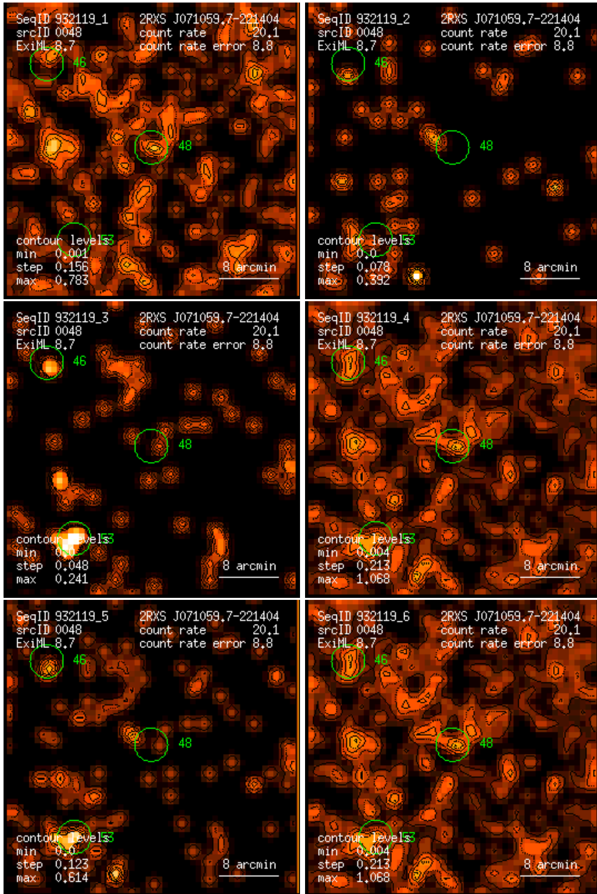
Figure 48: RASS 932119: detection 0048: band rate images, Gaussian filter: (1) PSPC channels 11 – 41, (2) 52 – 90, (3) 91 – 201, (4) 11 – 235, (5) 52 – 201, (6) 11 – 201. Broad band rates in counts/ks. Band rate contour levels in counts/ks/arcmin 2 .
