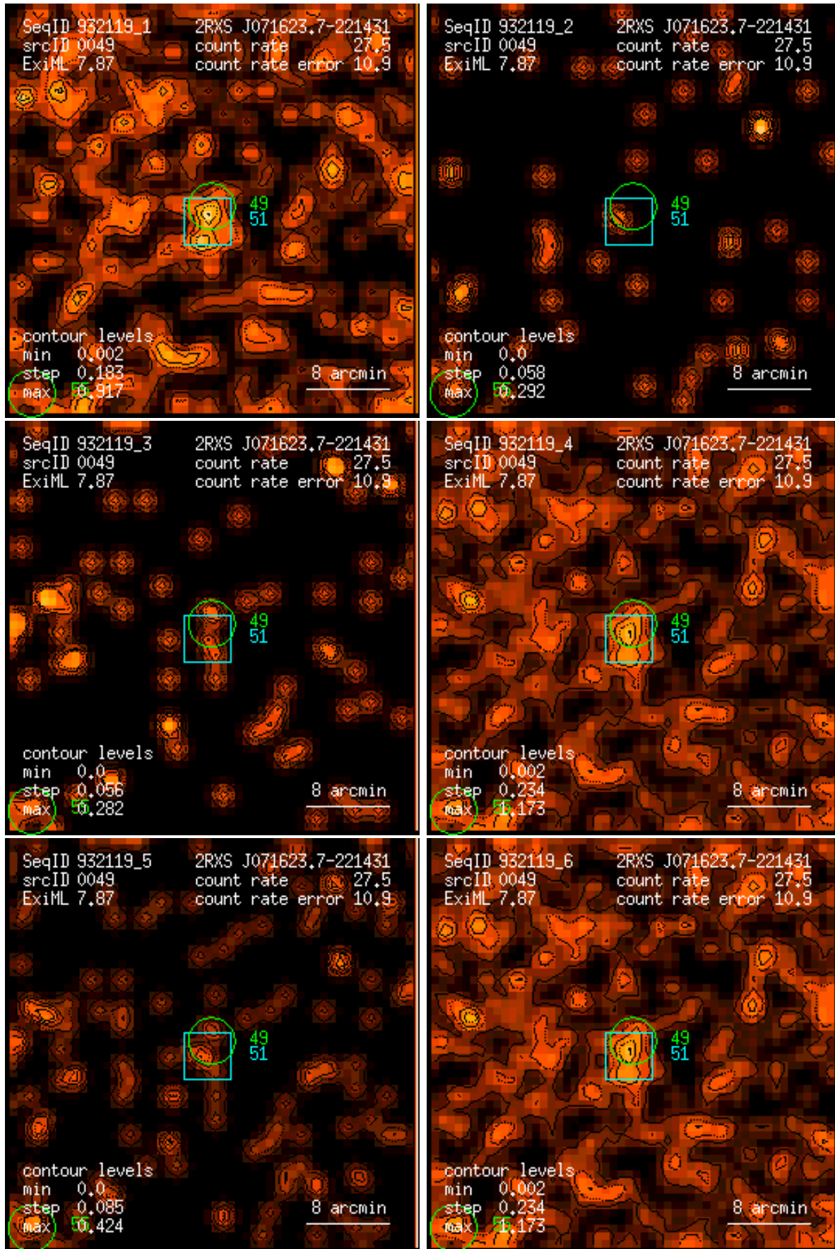
Figure 49: RASS 932119: detection 0049: band rate images, Gaussian filter: (1) PSPC channels 11 – 41, (2) 52 – 90, (3) 91 – 201, (4) 11 – 235, (5) 52 – 201, (6) 11 – 201. Broad band rates in counts/ks. Band rate contour levels in counts/ks/arcmin 2 .
