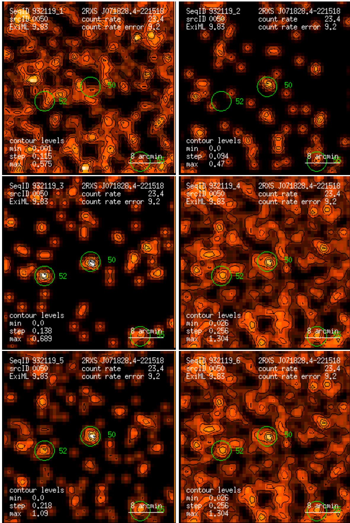
Figure 50: RASS 932119: detection 0050: band rate images, Gaussian filter: (1) PSPC channels 11 – 41, (2) 52 – 90, (3) 91 – 201, (4) 11 – 235, (5) 52 – 201, (6) 11 – 201. Broad band rates in counts/ks. Band rate contour levels in counts/ks/arcmin 2 .
