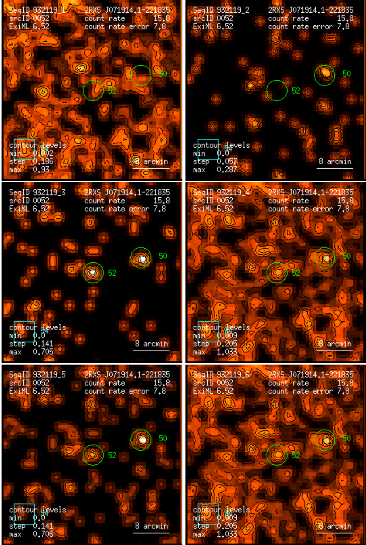
Figure 52: RASS 932119: detection 0052: band rate images, Gaussian filter: (1) PSPC channels 11 – 41, (2) 52 – 90, (3) 91 – 201, (4) 11 – 235, (5) 52 – 201, (6) 11 – 201. Broad band rates in counts/ks. Band rate contour levels in counts/ks/arcmin 2 .
