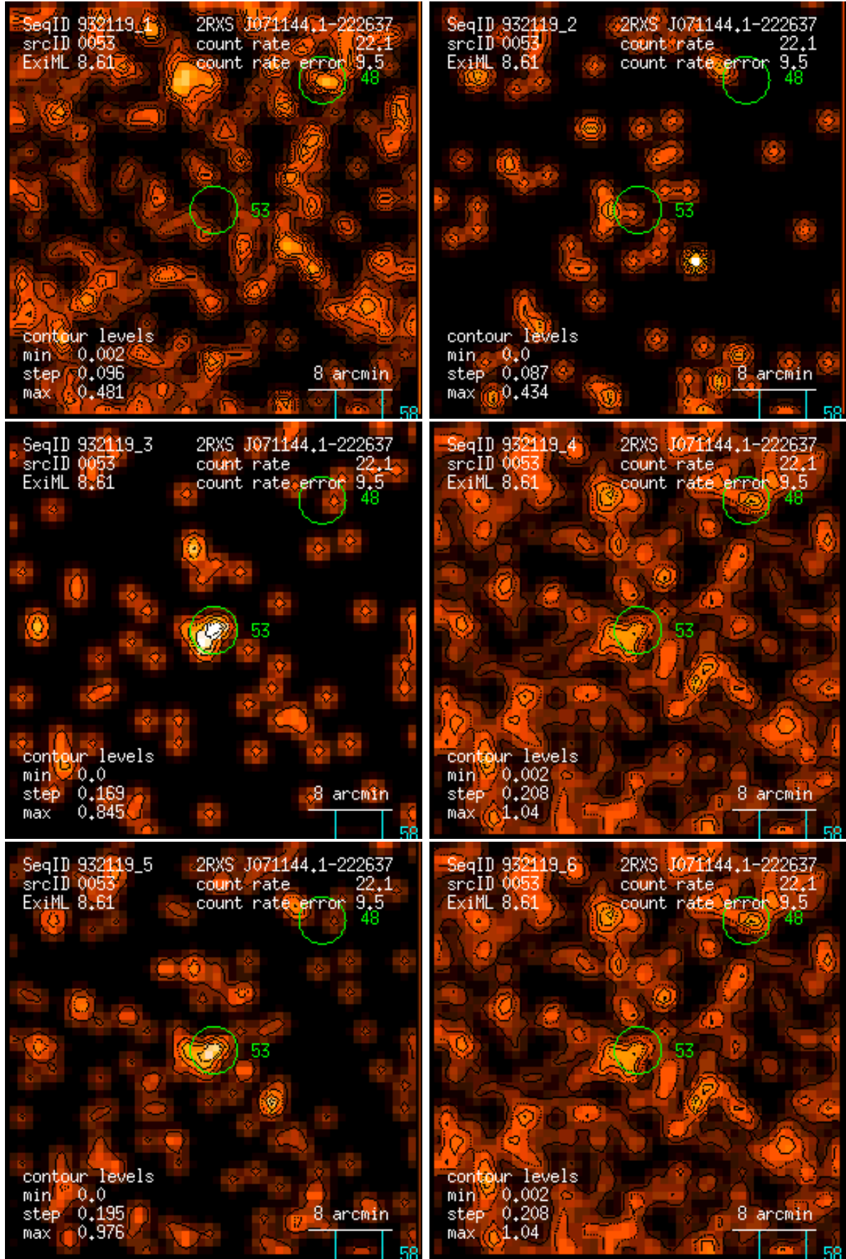
Figure 53: RASS 932119: detection 0053: band rate images, Gaussian filter: (1) PSPC channels 11 – 41, (2) 52 – 90, (3) 91 – 201, (4) 11 – 235, (5) 52 – 201, (6) 11 – 201. Broad band rates in counts/ks. Band rate contour levels in counts/ks/arcmin 2 .
