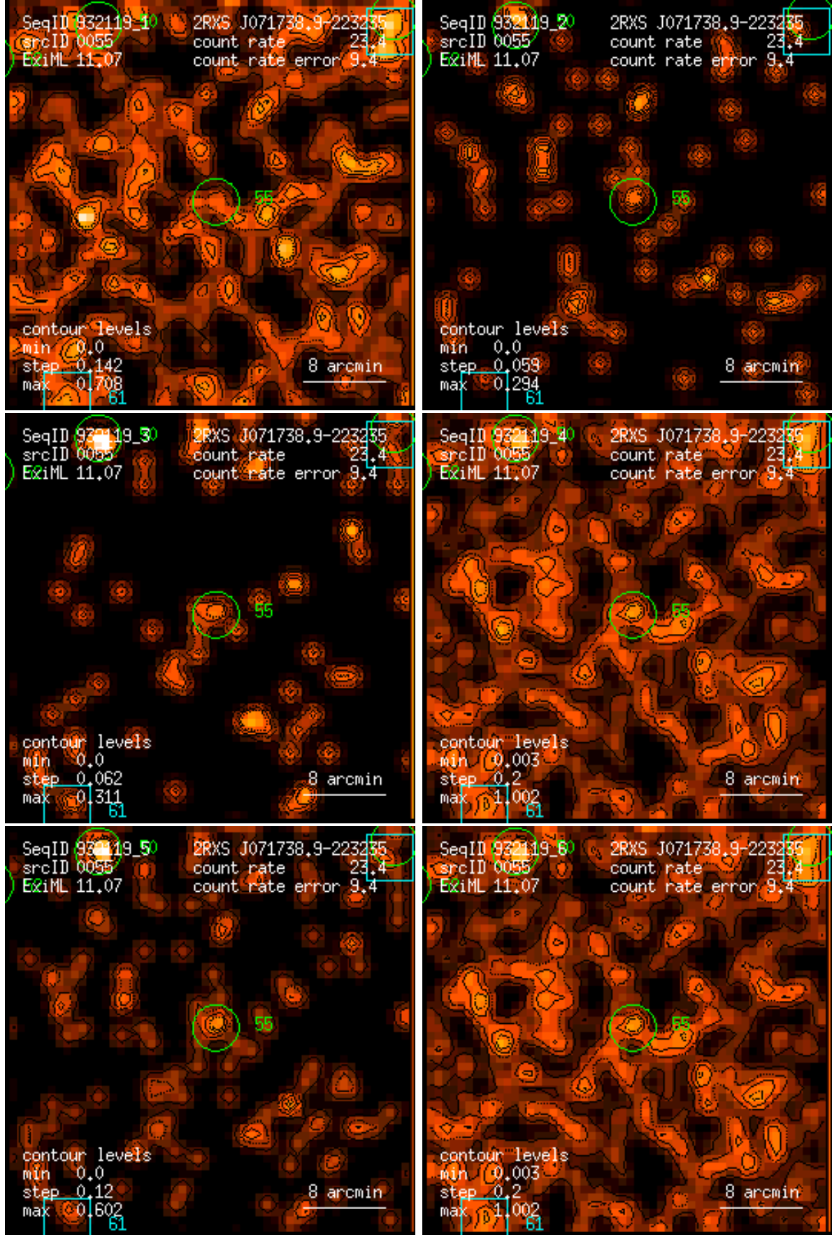
Figure 55: RASS 932119: detection 0055: band rate images, Gaussian filter: (1) PSPC channels 11 – 41, (2) 52 – 90, (3) 91 – 201, (4) 11 – 235, (5) 52 – 201, (6) 11 – 201. Broad band rates in counts/ks. Band rate contour levels in counts/ks/arcmin 2 .
