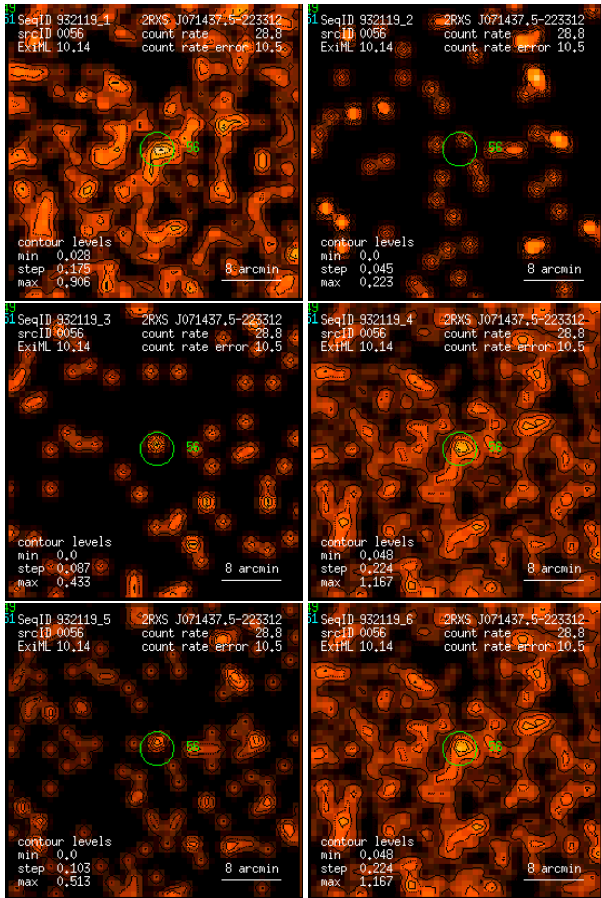
Figure 56: RASS 932119: detection 0056: band rate images, Gaussian filter: (1) PSPC channels 11 – 41, (2) 52 – 90, (3) 91 – 201, (4) 11 – 235, (5) 52 – 201, (6) 11 – 201. Broad band rates in counts/ks. Band rate contour levels in counts/ks/arcmin 2 .
