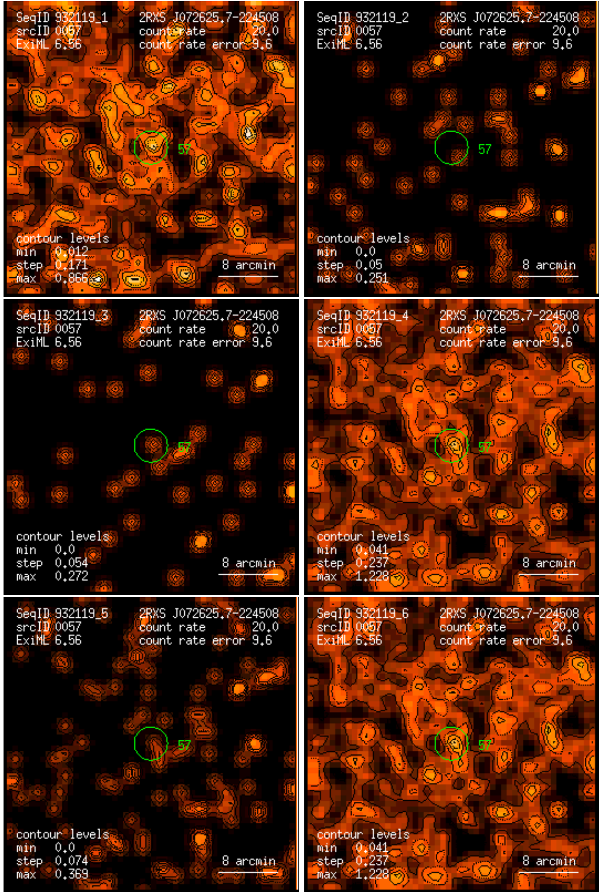
Figure 57: RASS 932119: detection 0057: band rate images, Gaussian filter: (1) PSPC channels 11 – 41, (2) 52 – 90, (3) 91 – 201, (4) 11 – 235, (5) 52 – 201, (6) 11 – 201. Broad band rates in counts/ks. Band rate contour levels in counts/ks/arcmin 2 .
