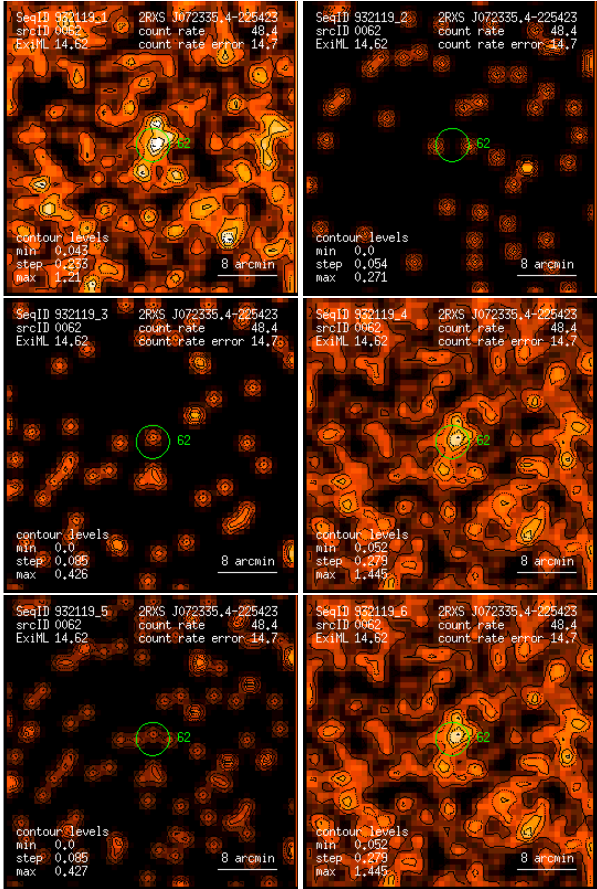
Figure 62: RASS 932119: detection 0062: band rate images, Gaussian filter: (1) PSPC channels 11 – 41, (2) 52 – 90, (3) 91 – 201, (4) 11 – 235, (5) 52 – 201, (6) 11 – 201. Broad band rates in counts/ks. Band rate contour levels in counts/ks/arcmin 2 .
