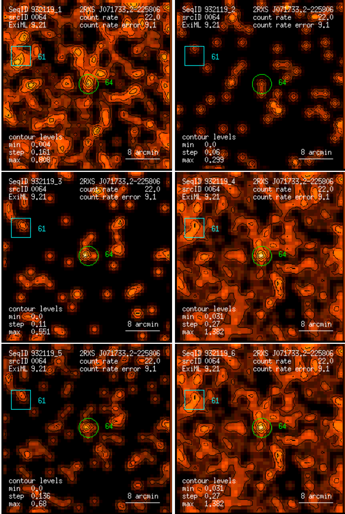
Figure 64: RASS 932119: detection 0064: band rate images, Gaussian filter: (1) PSPC channels 11 – 41, (2) 52 – 90, (3) 91 – 201, (4) 11 – 235, (5) 52 – 201, (6) 11 – 201. Broad band rates in counts/ks. Band rate contour levels in counts/ks/arcmin 2 .
