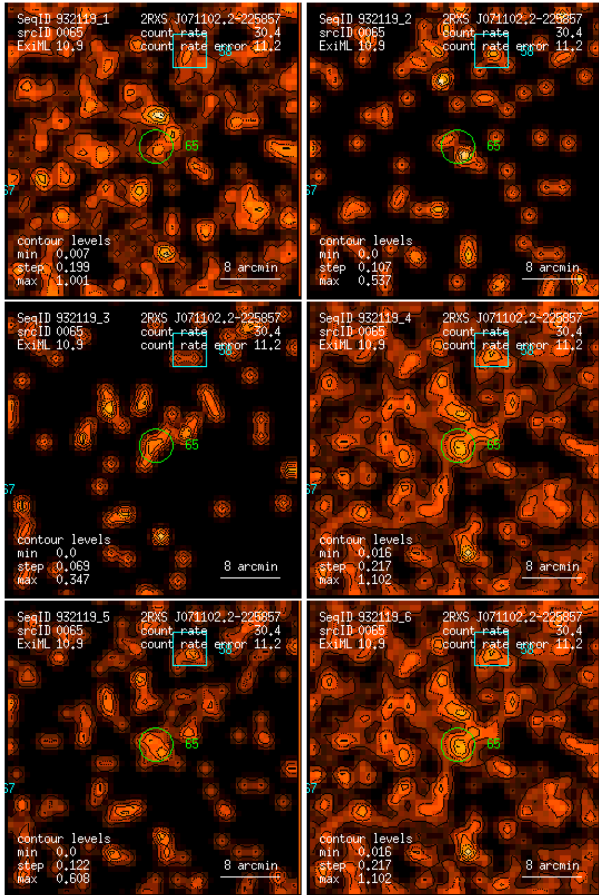
Figure 65: RASS 932119: detection 0065: band rate images, Gaussian filter: (1) PSPC channels 11 – 41, (2) 52 – 90, (3) 91 – 201, (4) 11 – 235, (5) 52 – 201, (6) 11 – 201. Broad band rates in counts/ks. Band rate contour levels in counts/ks/arcmin 2 .
