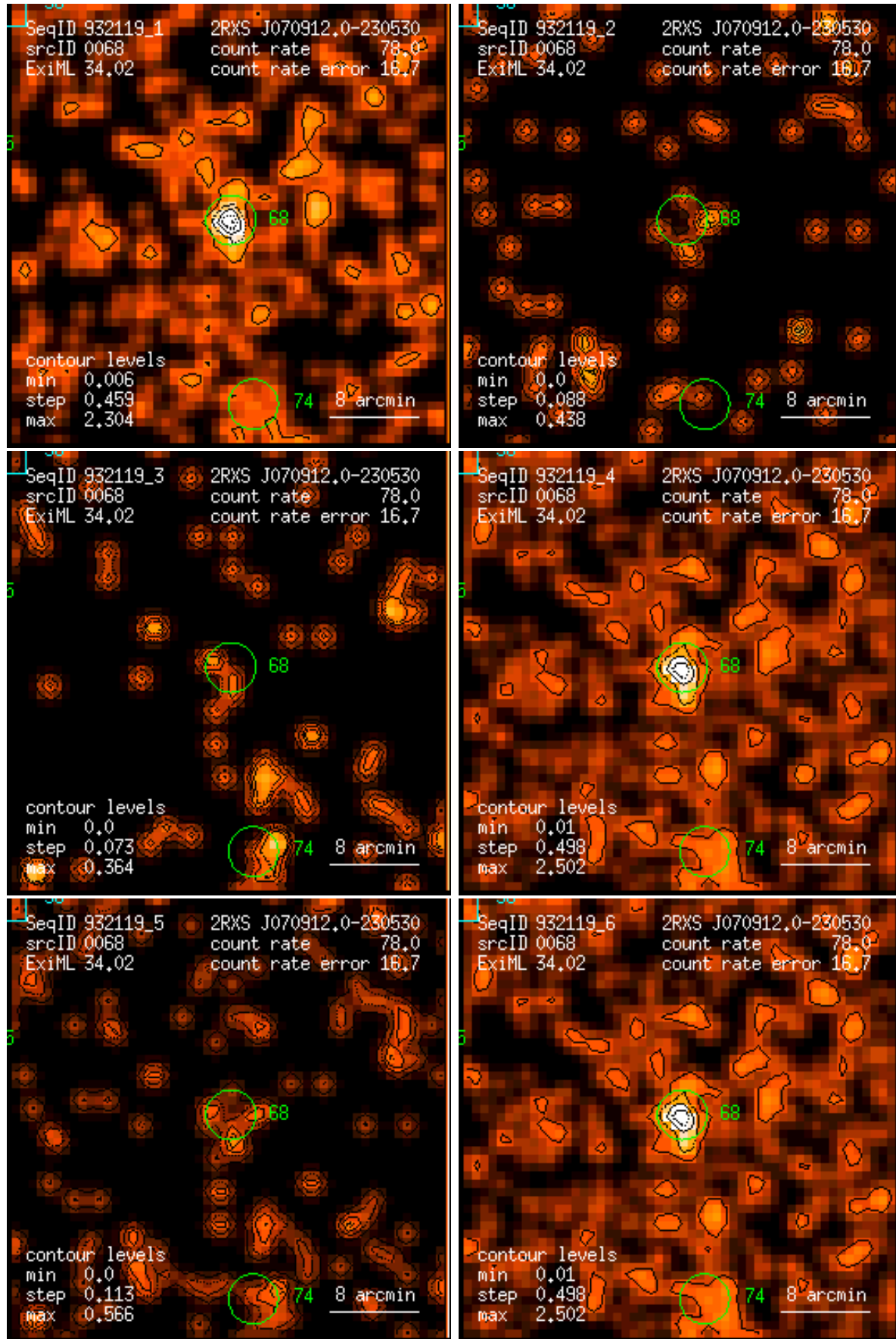
Figure 68: RASS 932119: detection 0068: band rate images, Gaussian filter: (1) PSPC channels 11 – 41, (2) 52 – 90, (3) 91 – 201, (4) 11 – 235, (5) 52 – 201, (6) 11 – 201. Broad band rates in counts/ks. Band rate contour levels in counts/ks/arcmin 2 .
