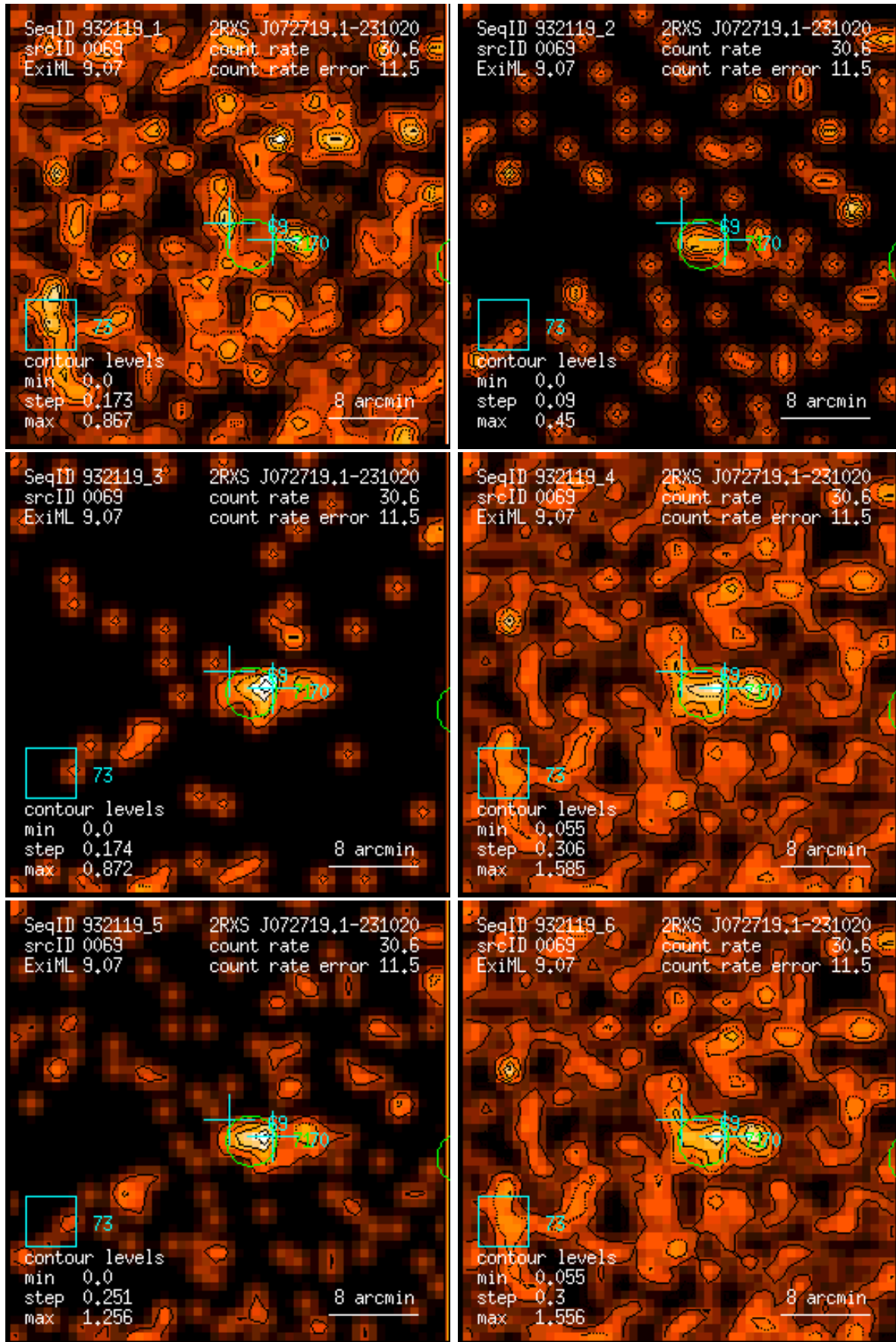
Figure 69: RASS 932119: detection 0069: band rate images, Gaussian filter: (1) PSPC channels 11 – 41, (2) 52 – 90, (3) 91 – 201, (4) 11 – 235, (5) 52 – 201, (6) 11 – 201. Broad band rates in counts/ks. Band rate contour levels in counts/ks/arcmin 2 .
