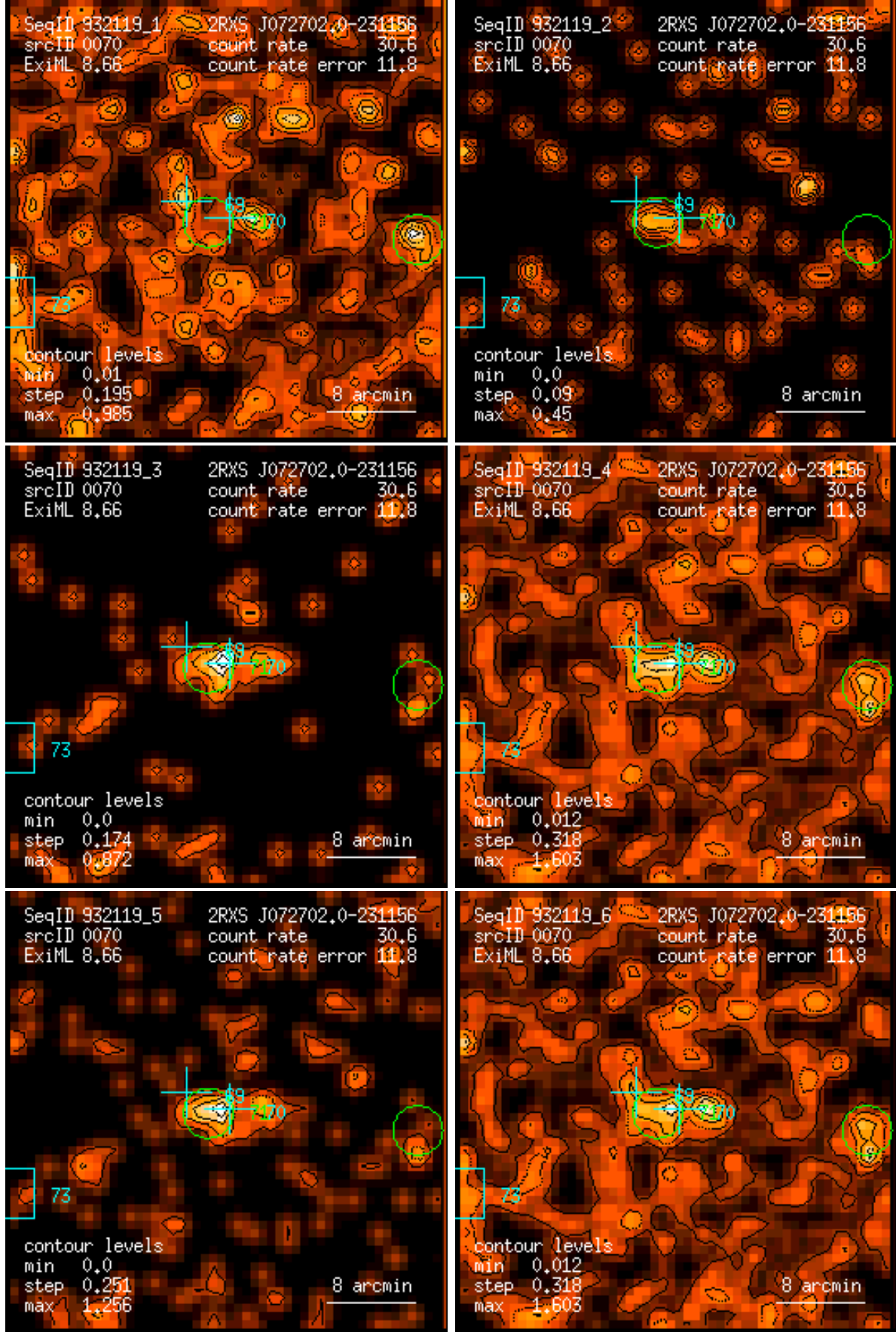
Figure 70: RASS 932119: detection 0070: band rate images, Gaussian filter: (1) PSPC channels 11 – 41, (2) 52 – 90, (3) 91 – 201, (4) 11 – 235, (5) 52 – 201, (6) 11 – 201. Broad band rates in counts/ks. Band rate contour levels in counts/ks/arcmin 2 .
