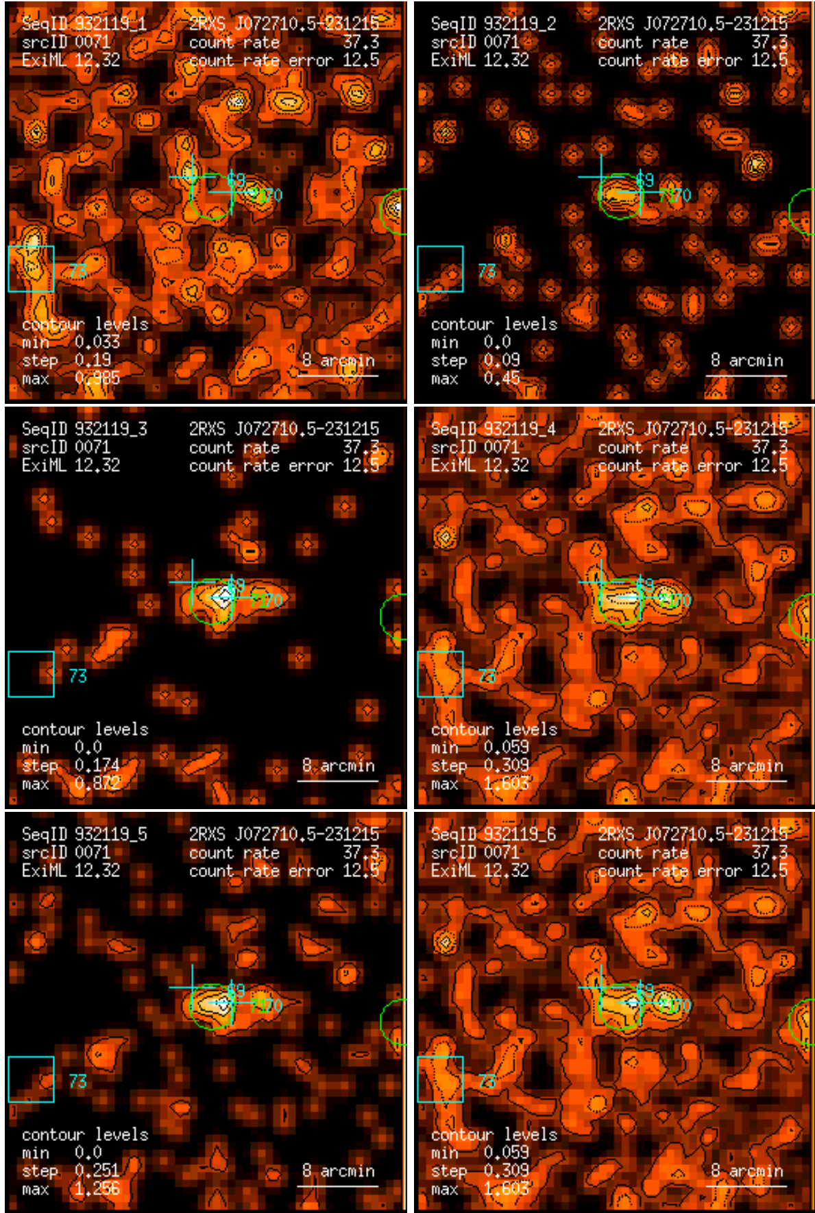
Figure 71: RASS 932119: detection 0071: band rate images, Gaussian filter: (1) PSPC channels 11 – 41, (2) 52 – 90, (3) 91 – 201, (4) 11 – 235, (5) 52 – 201, (6) 11 – 201. Broad band rates in counts/ks. Band rate contour levels in counts/ks/arcmin 2 .
