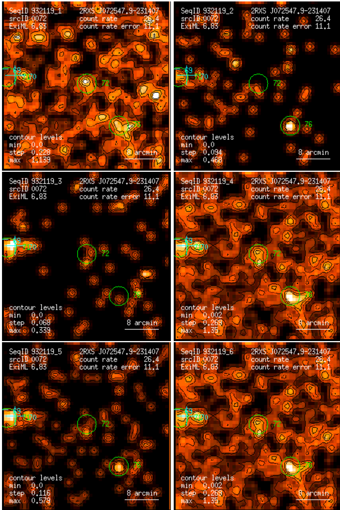
Figure 72: RASS 932119: detection 0072: band rate images, Gaussian filter: (1) PSPC channels 11 – 41, (2) 52 – 90, (3) 91 – 201, (4) 11 – 235, (5) 52 – 201, (6) 11 – 201. Broad band rates in counts/ks. Band rate contour levels in counts/ks/arcmin 2 .
