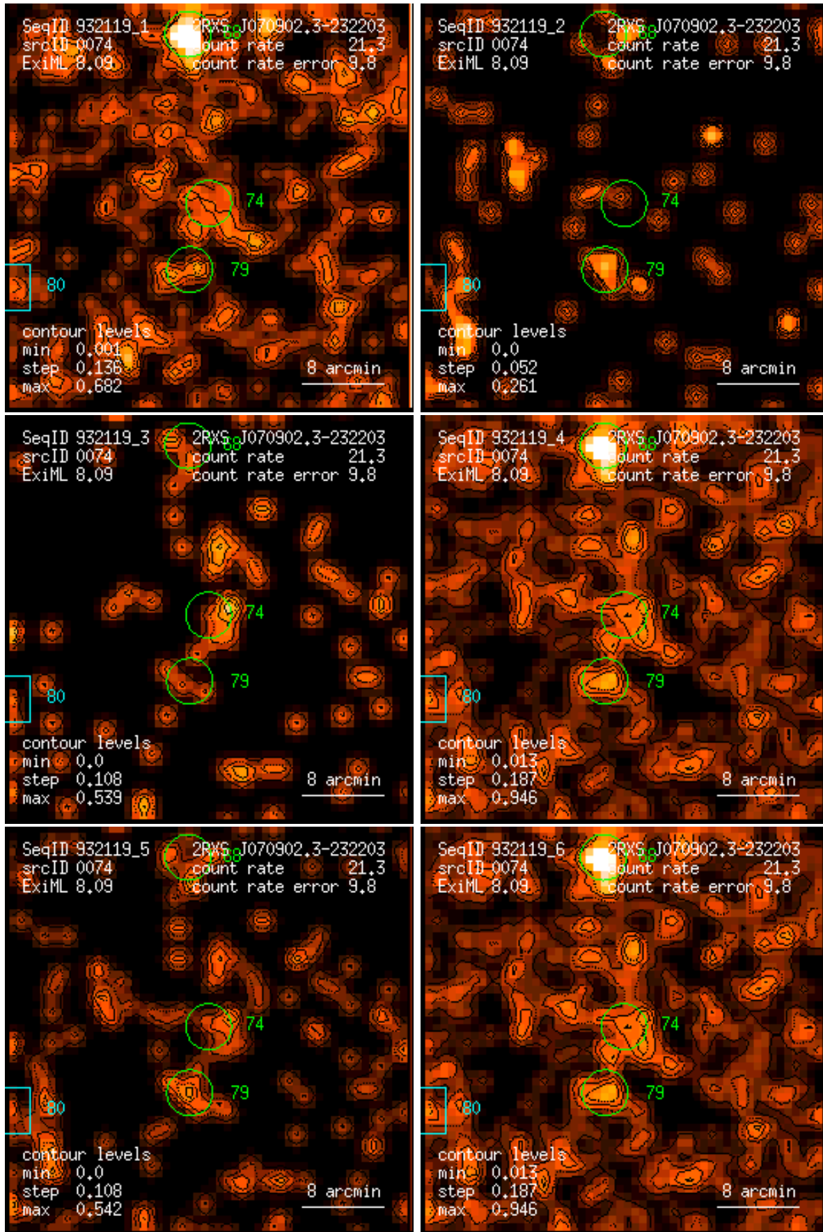
Figure 74: RASS 932119: detection 0074: band rate images, Gaussian filter: (1) PSPC channels 11 – 41, (2) 52 – 90, (3) 91 – 201, (4) 11 – 235, (5) 52 – 201, (6) 11 – 201. Broad band rates in counts/ks. Band rate contour levels in counts/ks/arcmin 2 .
