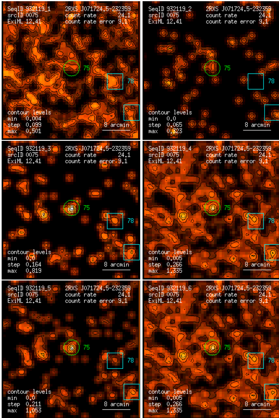
Figure 75: RASS 932119: detection 0075: band rate images, Gaussian filter: (1) PSPC channels 11 – 41, (2) 52 – 90, (3) 91 – 201, (4) 11 – 235, (5) 52 – 201, (6) 11 – 201. Broad band rates in counts/ks. Band rate contour levels in counts/ks/arcmin 2 .
