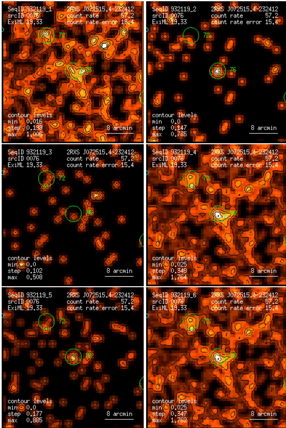
Figure 76: RASS 932119: detection 0076: band rate images, Gaussian filter: (1) PSPC channels 11 – 41, (2) 52 – 90, (3) 91 – 201, (4) 11 – 235, (5) 52 – 201, (6) 11 – 201. Broad band rates in counts/ks. Band rate contour levels in counts/ks/arcmin 2 .
