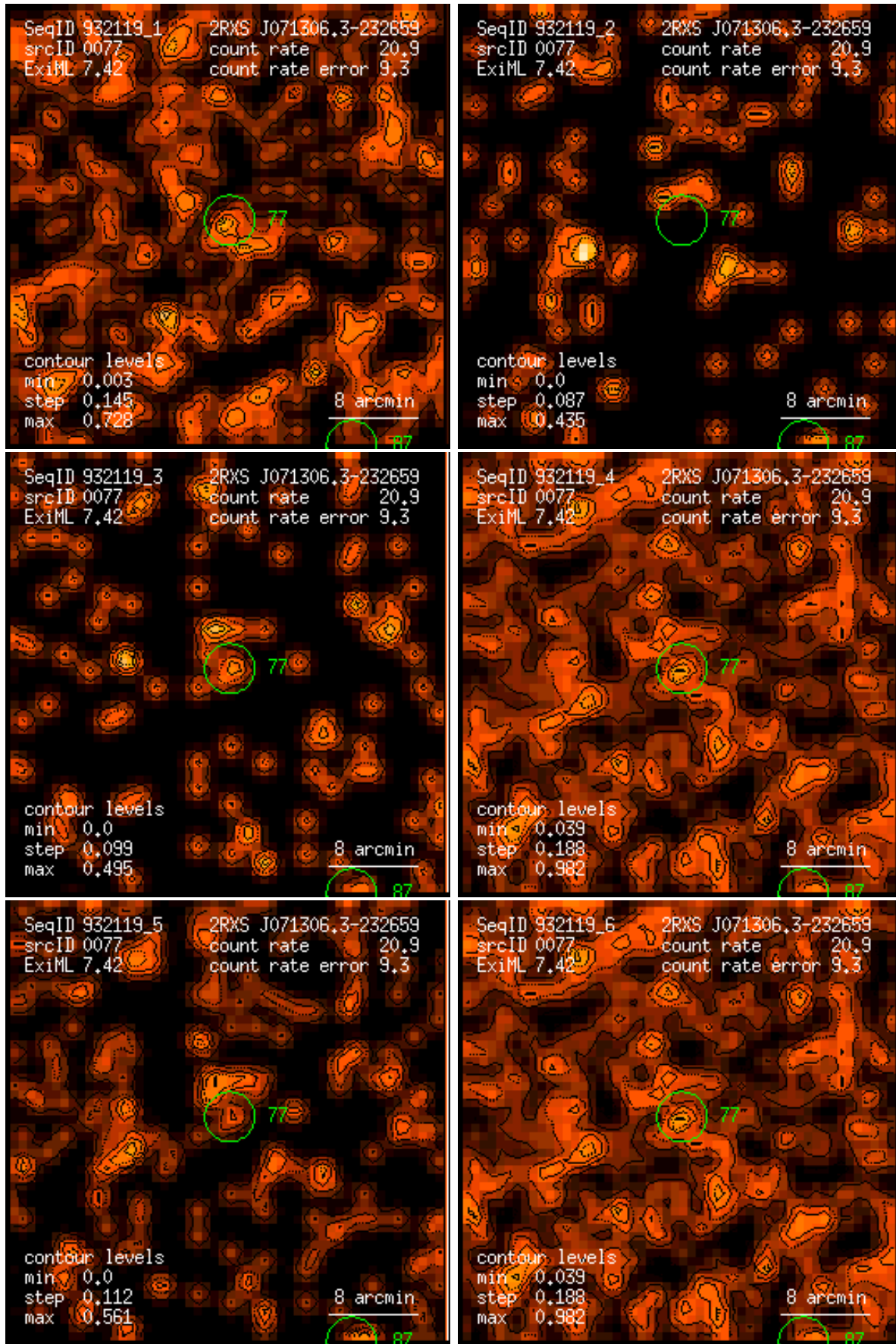
Figure 77: RASS 932119: detection 0077: band rate images, Gaussian filter: (1) PSPC channels 11 – 41, (2) 52 – 90, (3) 91 – 201, (4) 11 – 235, (5) 52 – 201, (6) 11 – 201. Broad band rates in counts/ks. Band rate contour levels in counts/ks/arcmin 2 .
