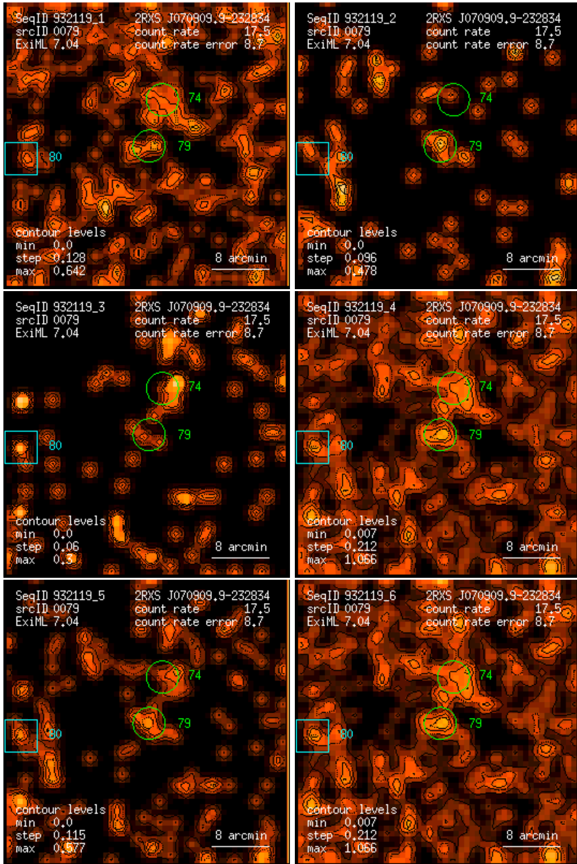
Figure 79: RASS 932119: detection 0079: band rate images, Gaussian filter: (1) PSPC channels 11 – 41, (2) 52 – 90, (3) 91 – 201, (4) 11 – 235, (5) 52 – 201, (6) 11 – 201. Broad band rates in counts/ks. Band rate contour levels in counts/ks/arcmin 2 .
