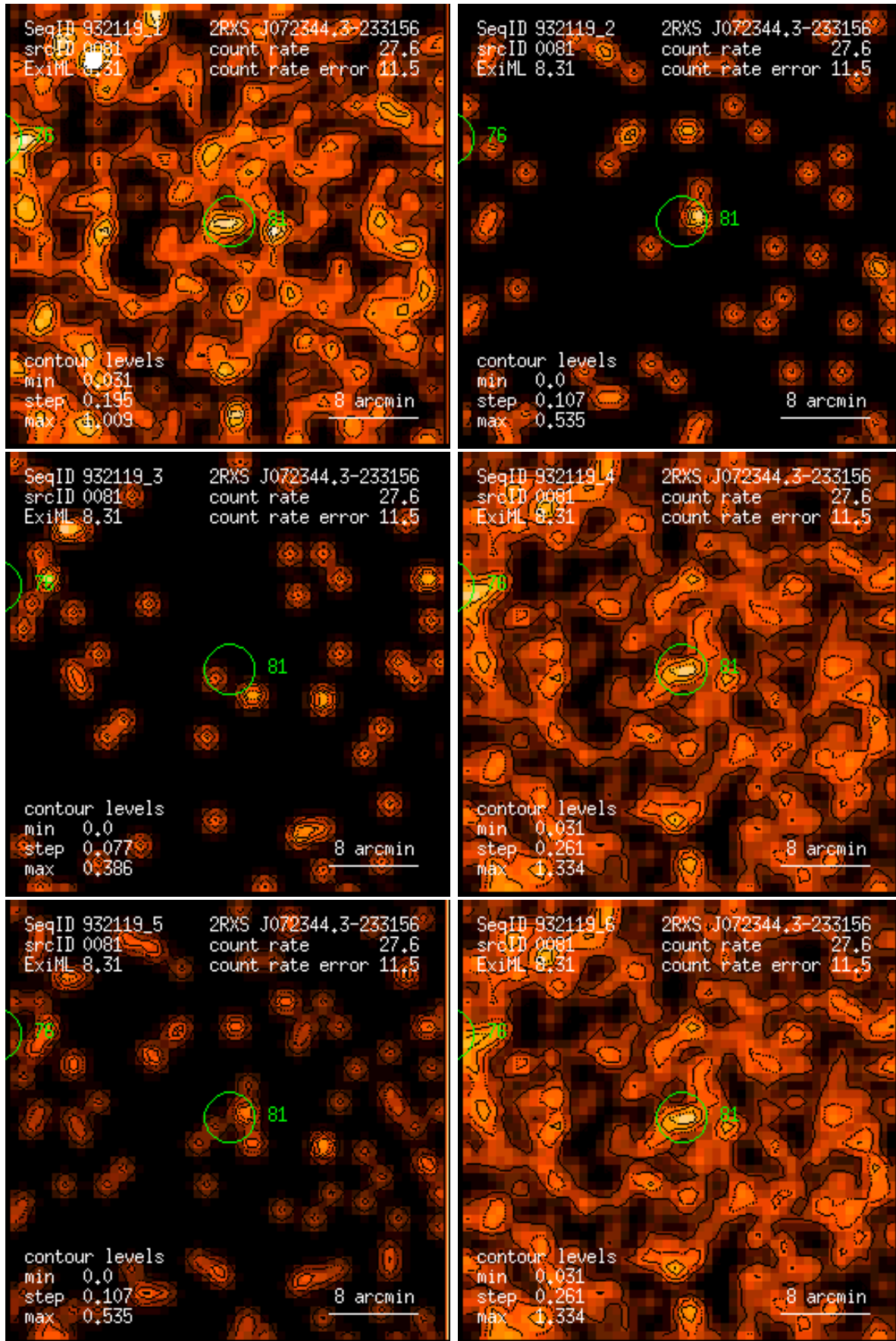
Figure 81: RASS 932119: detection 0081: band rate images, Gaussian filter: (1) PSPC channels 11 – 41, (2) 52 – 90, (3) 91 – 201, (4) 11 – 235, (5) 52 – 201, (6) 11 – 201. Broad band rates in counts/ks. Band rate contour levels in counts/ks/arcmin 2 .
