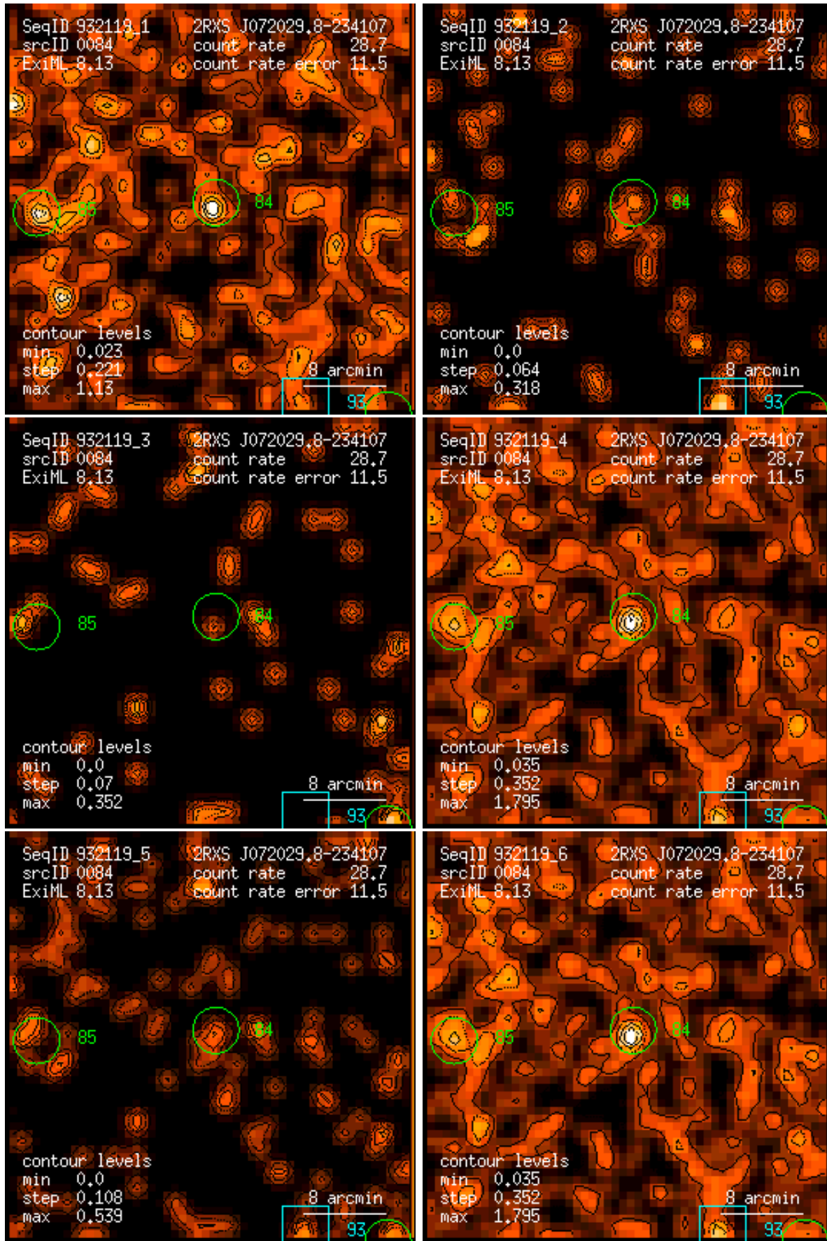
Figure 84: RASS 932119: detection 0084: band rate images, Gaussian filter: (1) PSPC channels 11 – 41, (2) 52 – 90, (3) 91 – 201, (4) 11 – 235, (5) 52 – 201, (6) 11 – 201. Broad band rates in counts/ks. Band rate contour levels in counts/ks/arcmin 2 .
