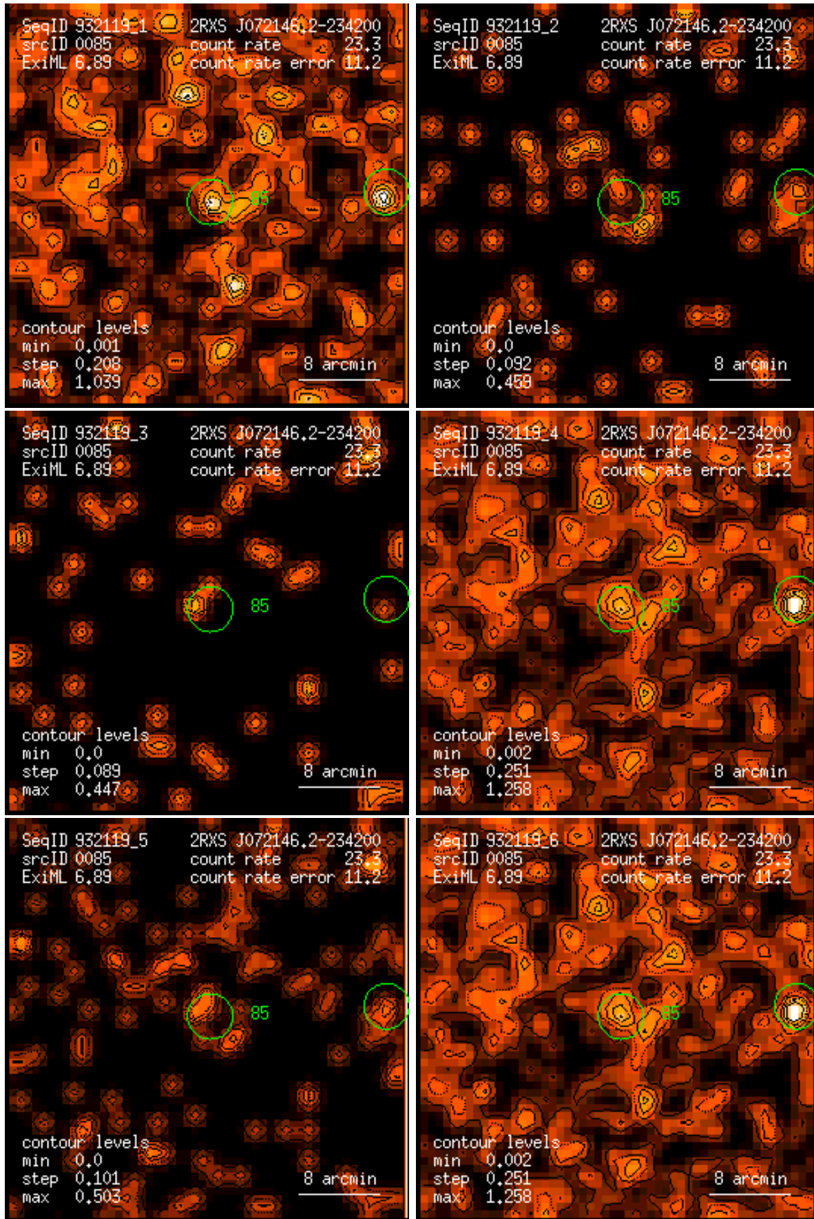
Figure 85: RASS 932119: detection 0085: band rate images, Gaussian filter: (1) PSPC channels 11 – 41, (2) 52 – 90, (3) 91 – 201, (4) 11 – 235, (5) 52 – 201, (6) 11 – 201. Broad band rates in counts/ks. Band rate contour levels in counts/ks/arcmin 2 .
