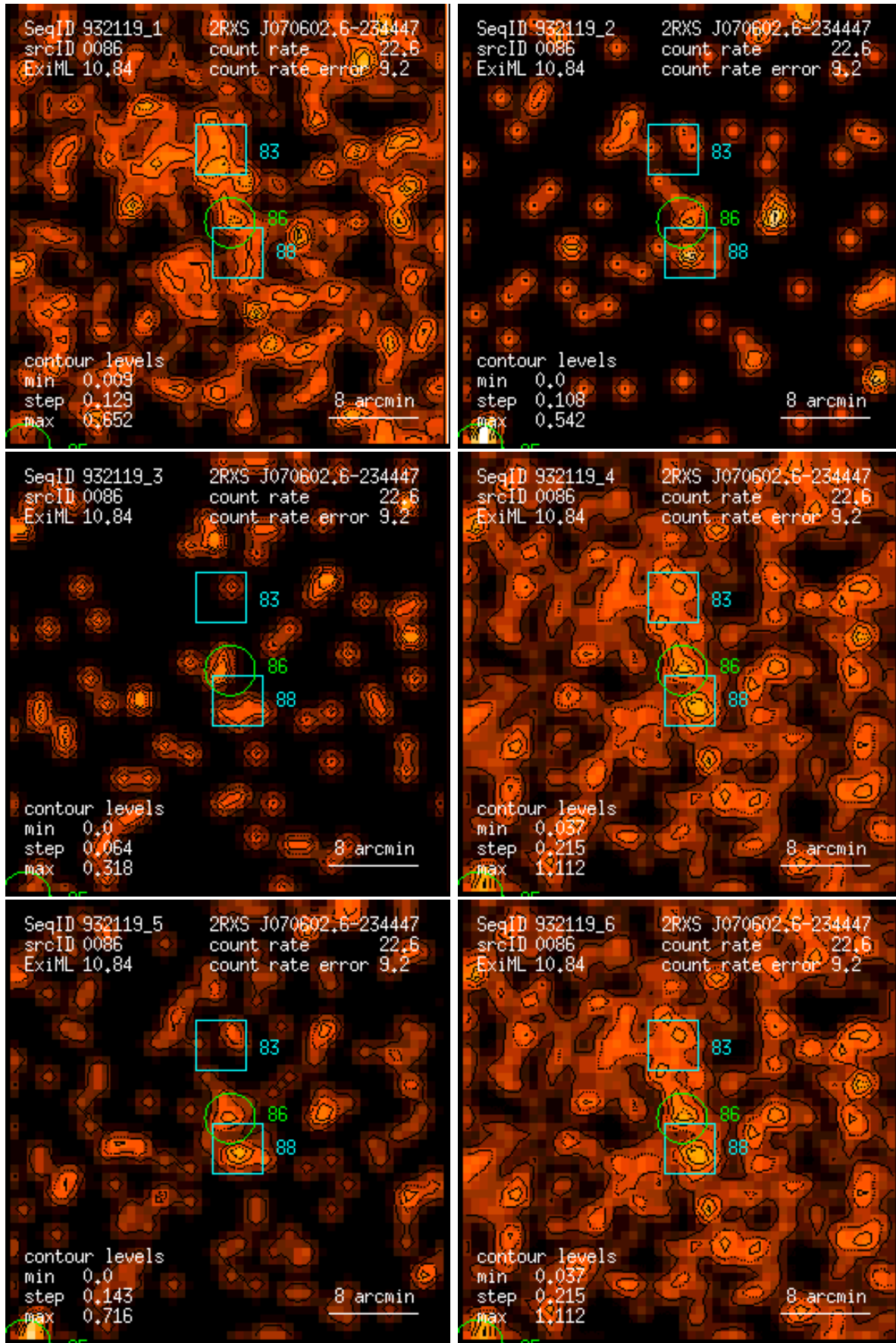
Figure 86: RASS 932119: detection 0086: band rate images, Gaussian filter: (1) PSPC channels 11 – 41, (2) 52 – 90, (3) 91 – 201, (4) 11 – 235, (5) 52 – 201, (6) 11 – 201. Broad band rates in counts/ks. Band rate contour levels in counts/ks/arcmin 2 .
